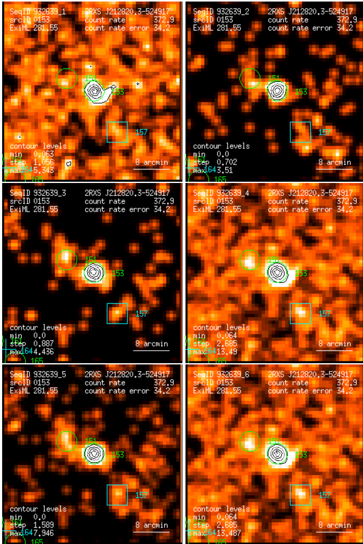
Figure 153: RASS 932639: detection 0153: band rate images, Gaussian filter: (1) PSPC channels 11 – 41, (2) 52 – 90, (3) 91 – 201, (4) 11 – 235, (5) 52 – 201, (6) 11 – 201. Broad band rates in counts/ks. Band rate contour levels in counts/ks/arcmin 2 .
