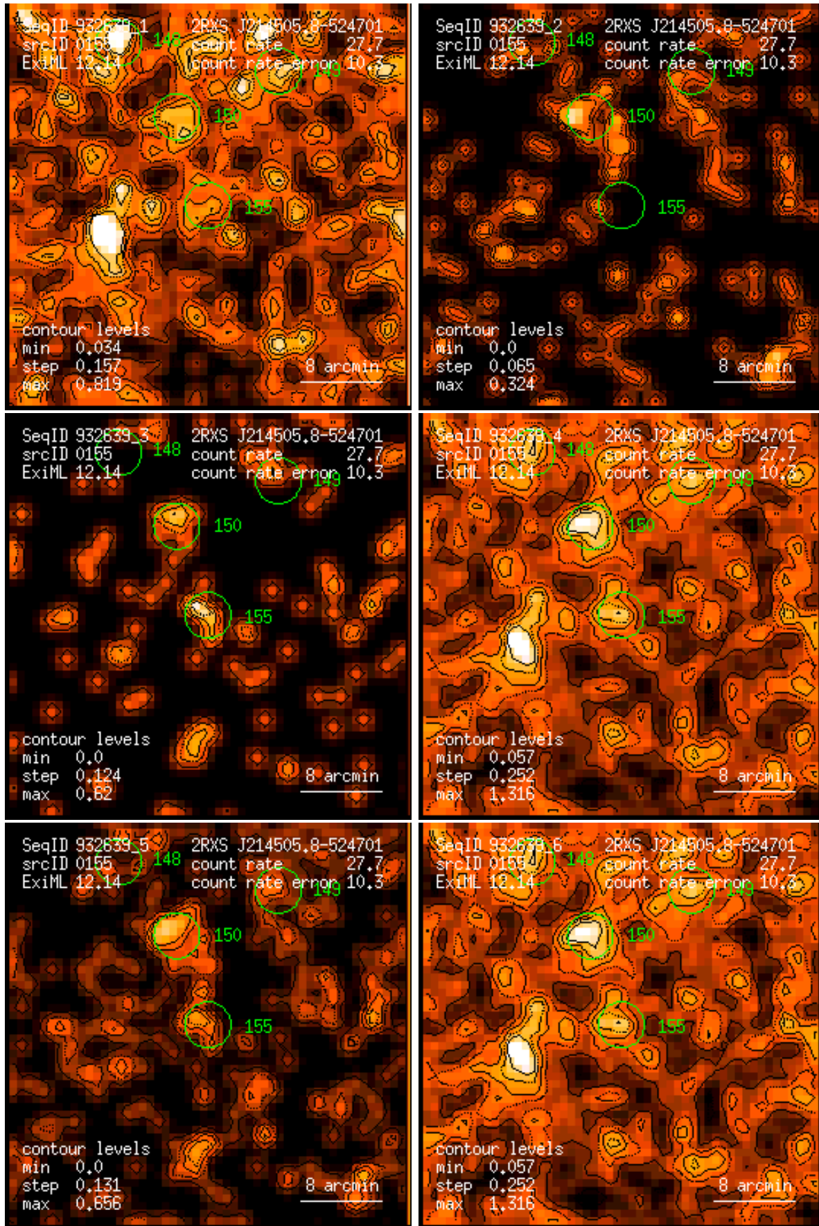
Figure 155: RASS 932639: detection 0155: band rate images, Gaussian filter: (1) PSPC channels 11 – 41, (2) 52 – 90, (3) 91 – 201, (4) 11 – 235, (5) 52 – 201, (6) 11 – 201. Broad band rates in counts/ks. Band rate contour levels in counts/ks/arcmin 2 .
