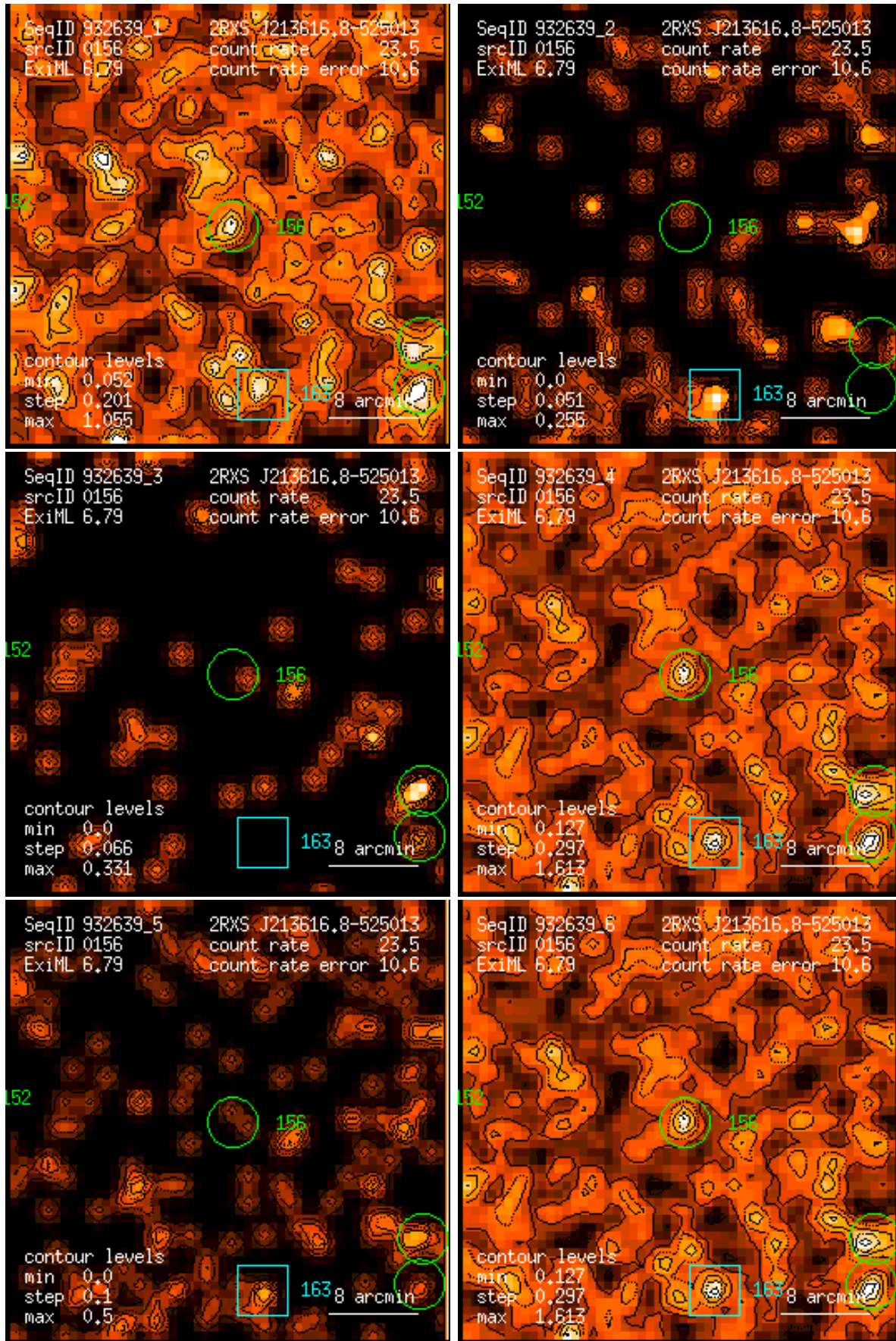
Figure 156: RASS 932639: detection 0156: band rate images, Gaussian filter: (1) PSPC channels 11 – 41, (2) 52 – 90, (3) 91 – 201, (4) 11 – 235, (5) 52 – 201, (6) 11 – 201. Broad band rates in counts/ks. Band rate contour levels in counts/ks/arcmin 2 .
