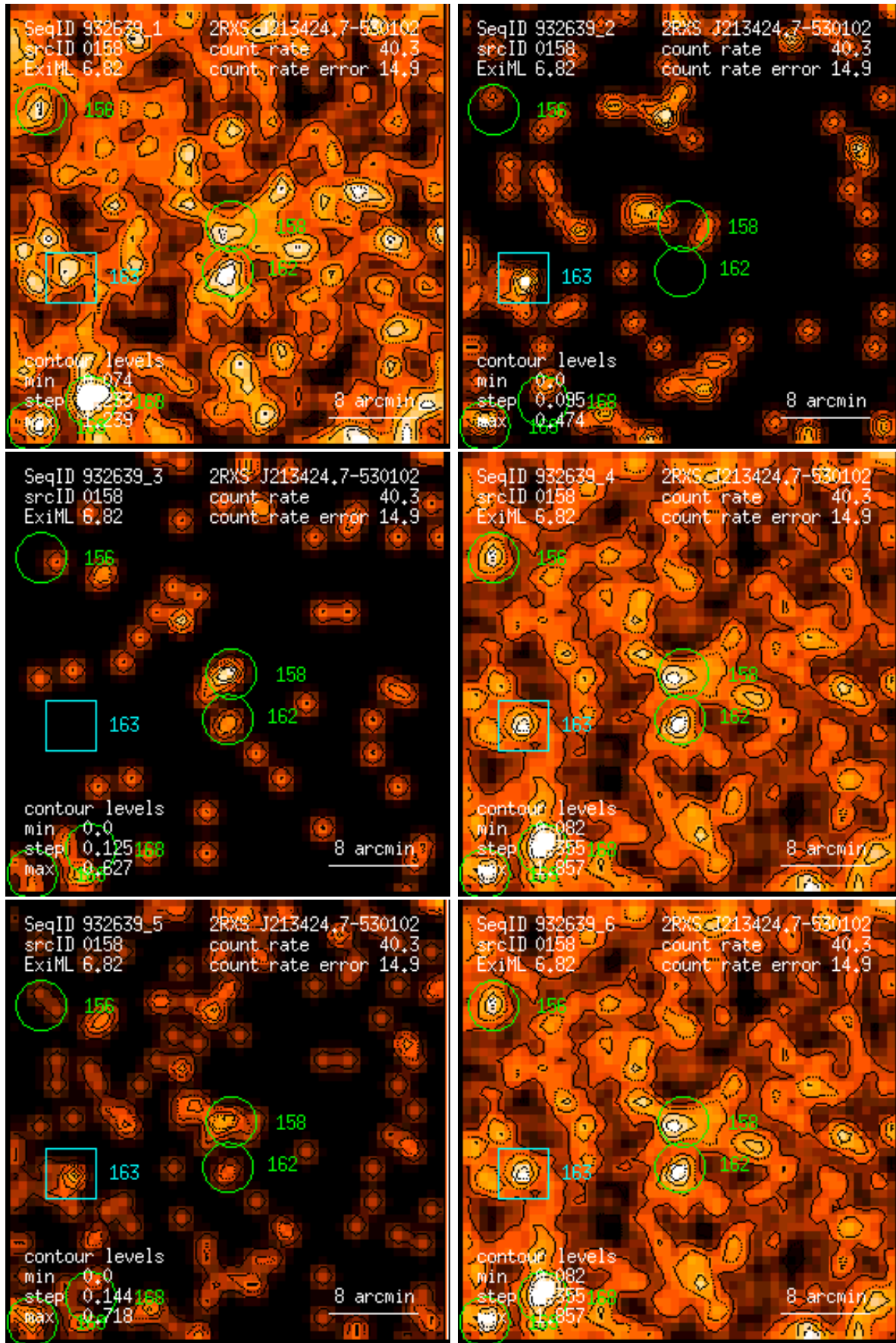
Figure 158: RASS 932639: detection 0158: band rate images, Gaussian filter: (1) PSPC channels 11 – 41, (2) 52 – 90, (3) 91 – 201, (4) 11 – 235, (5) 52 – 201, (6) 11 – 201. Broad band rates in counts/ks. Band rate contour levels in counts/ks/arcmin 2 .
