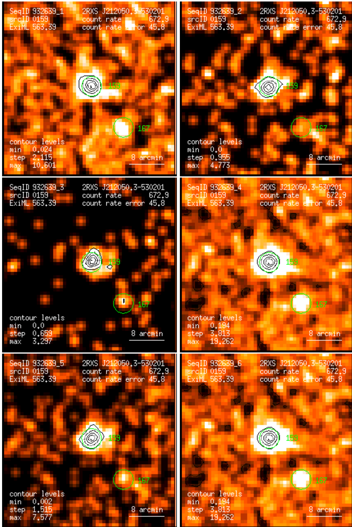
Figure 159: RASS 932639: detection 0159: band rate images, Gaussian filter: (1) PSPC channels 11 – 41, (2) 52 – 90, (3) 91 – 201, (4) 11 – 235, (5) 52 – 201, (6) 11 – 201. Broad band rates in counts/ks. Band rate contour levels in counts/ks/arcmin 2 .
