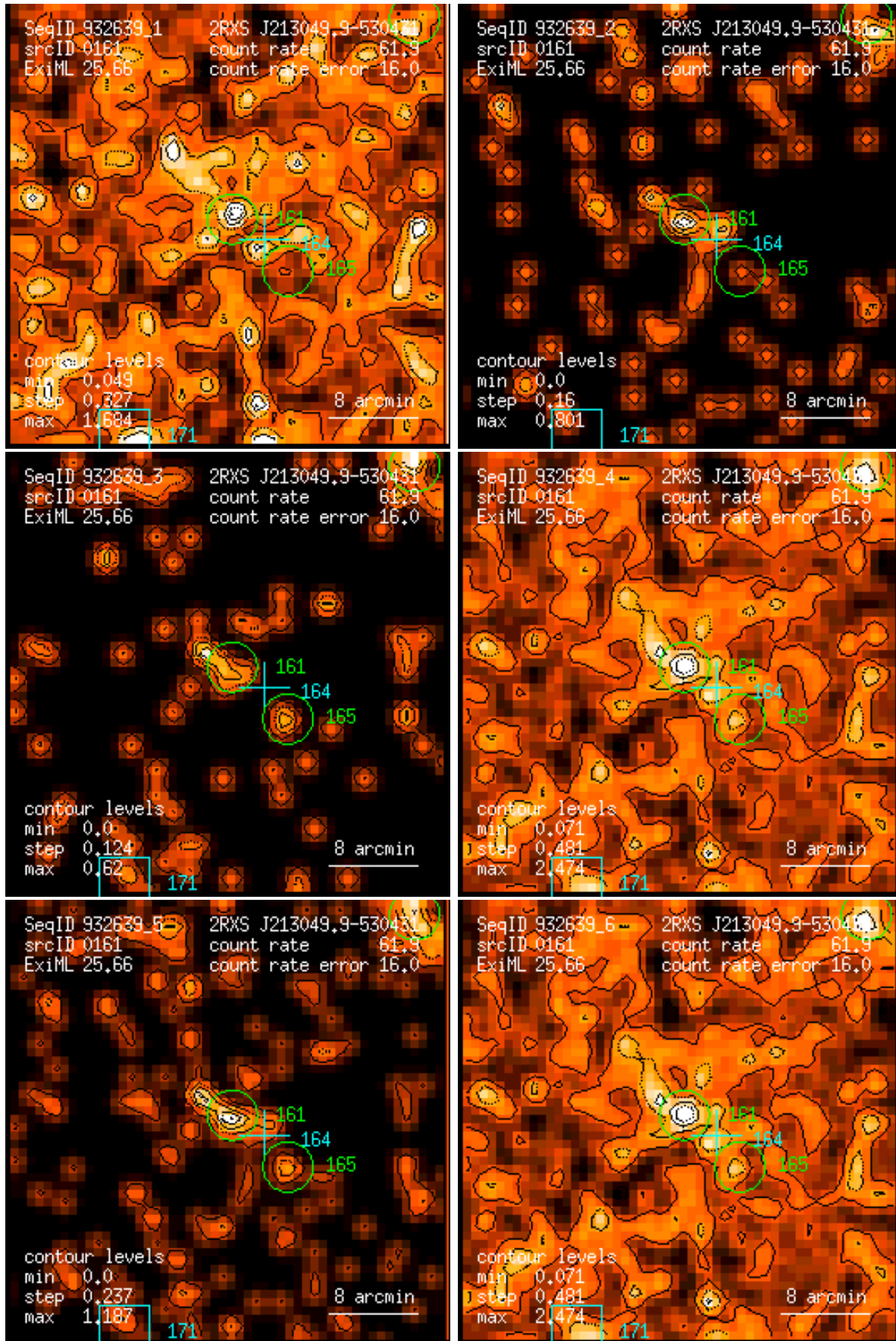
Figure 161: RASS 932639: detection 0161: band rate images, Gaussian filter: (1) PSPC channels 11 – 41, (2) 52 – 90, (3) 91 – 201, (4) 11 – 235, (5) 52 – 201, (6) 11 – 201. Broad band rates in counts/ks. Band rate contour levels in counts/ks/arcmin 2 .
