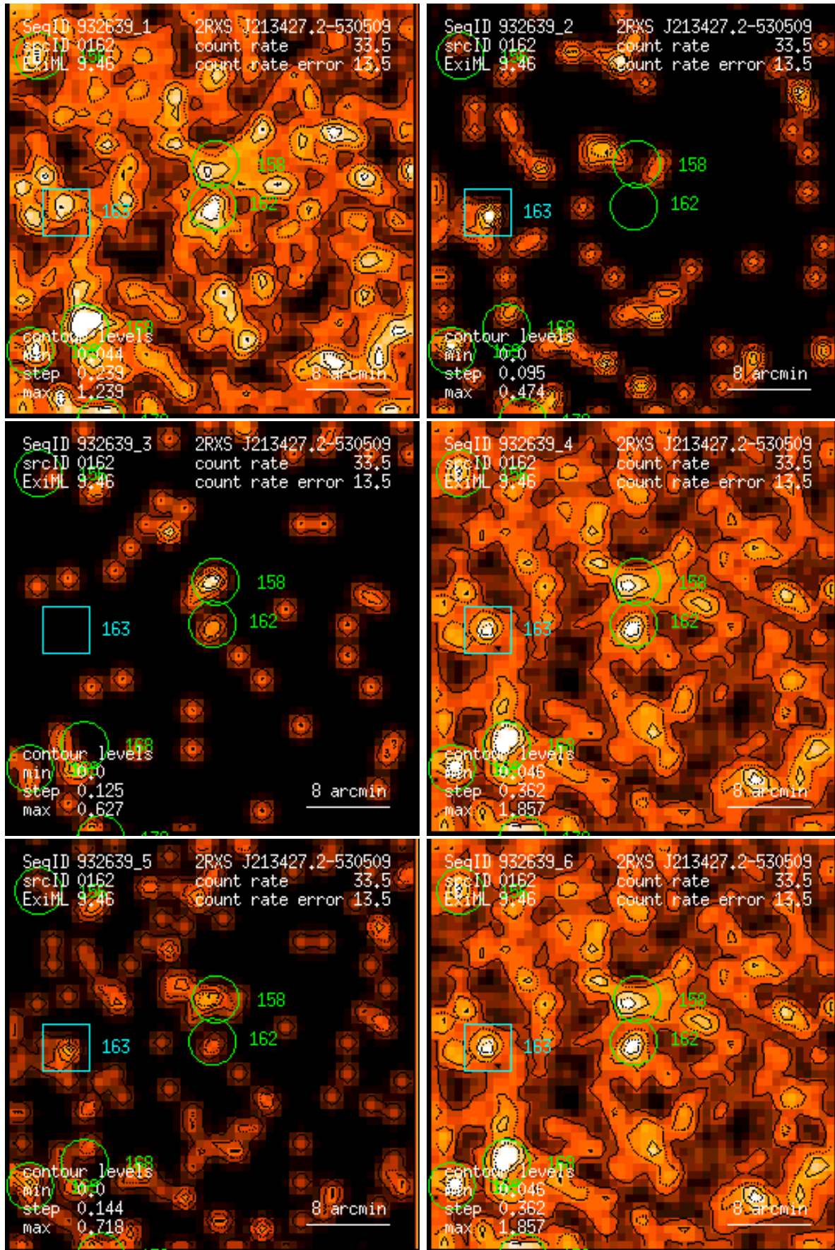
Figure 162: RASS 932639: detection 0162: band rate images, Gaussian filter: (1) PSPC channels 11 – 41, (2) 52 – 90, (3) 91 – 201, (4) 11 – 235, (5) 52 – 201, (6) 11 – 201. Broad band rates in counts/ks. Band rate contour levels in counts/ks/arcmin 2 .
