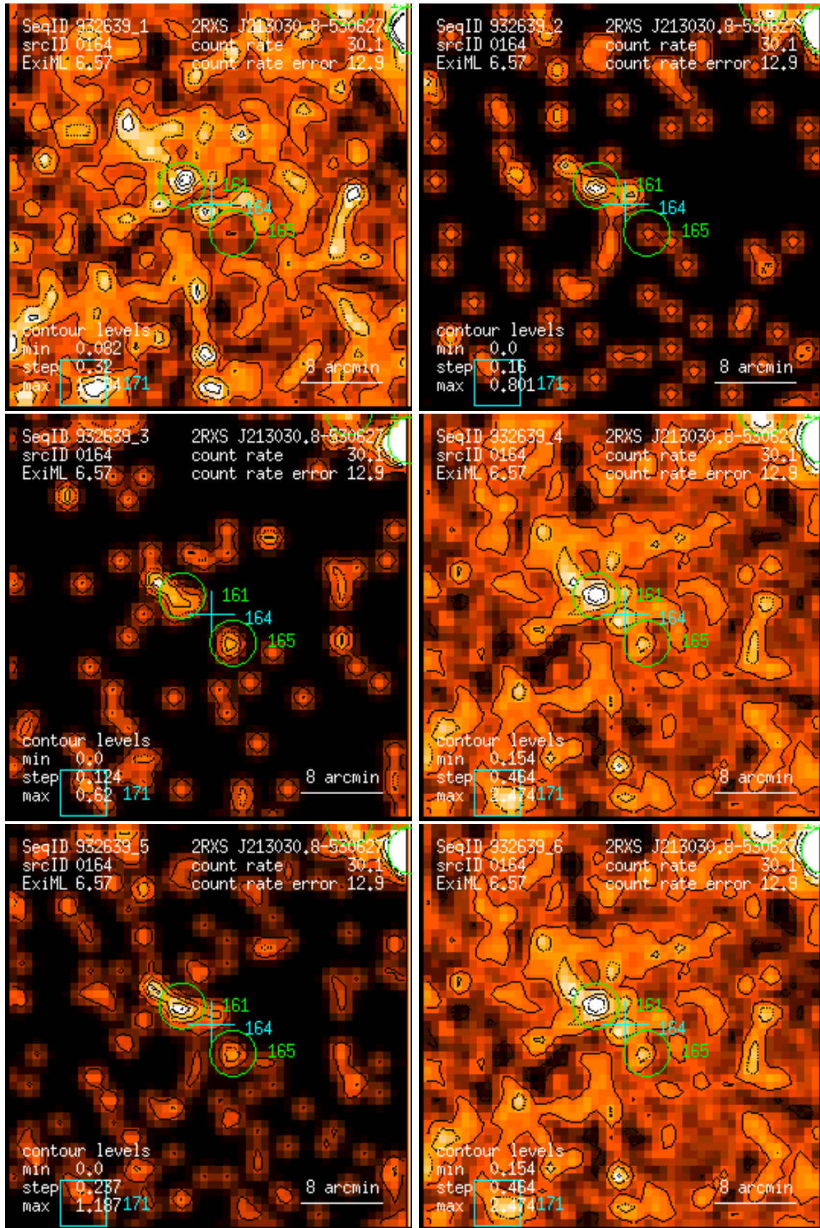
Figure 164: RASS 932639: detection 0164: band rate images, Gaussian filter: (1) PSPC channels 11 – 41, (2) 52 – 90, (3) 91 – 201, (4) 11 – 235, (5) 52 – 201, (6) 11 – 201. Broad band rates in counts/ks. Band rate contour levels in counts/ks/arcmin 2 .
