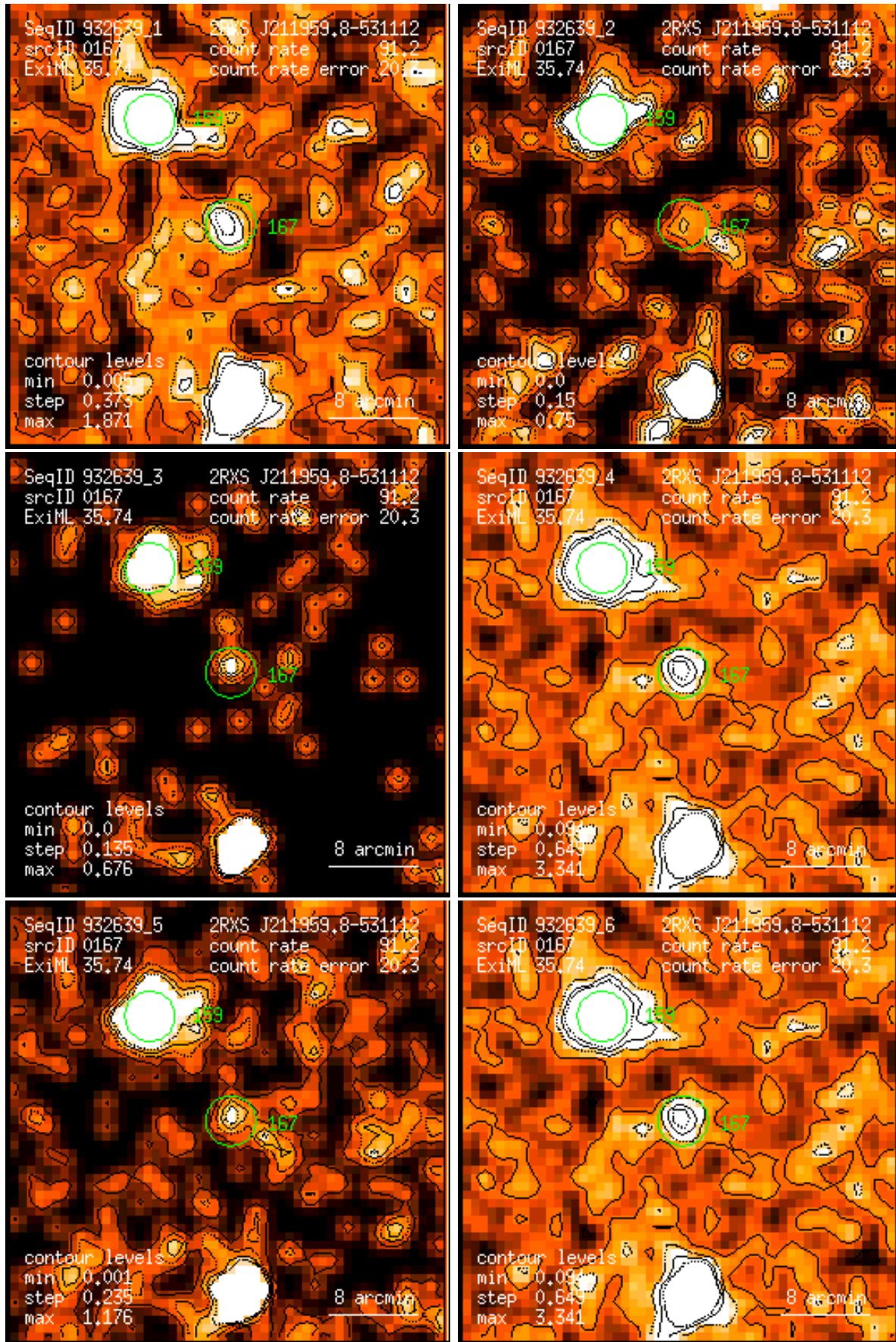
Figure 167: RASS 932639: detection 0167: band rate images, Gaussian filter: (1) PSPC channels 11 – 41, (2) 52 – 90, (3) 91 – 201, (4) 11 – 235, (5) 52 – 201, (6) 11 – 201. Broad band rates in counts/ks. Band rate contour levels in counts/ks/arcmin 2 .
