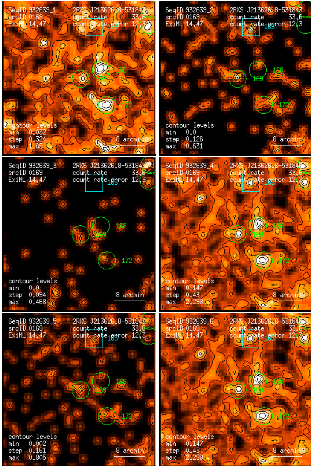
Figure 169: RASS 932639: detection 0169: band rate images, Gaussian filter: (1) PSPC channels 11 – 41, (2) 52 – 90, (3) 91 – 201, (4) 11 – 235, (5) 52 – 201, (6) 11 – 201. Broad band rates in counts/ks. Band rate contour levels in counts/ks/arcmin 2 .
