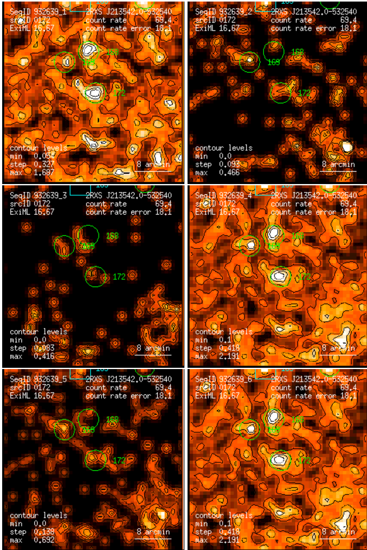
Figure 172: RASS 932639: detection 0172: band rate images, Gaussian filter: (1) PSPC channels 11 – 41, (2) 52 – 90, (3) 91 – 201, (4) 11 – 235, (5) 52 – 201, (6) 11 – 201. Broad band rates in counts/ks. Band rate contour levels in counts/ks/arcmin 2 .
