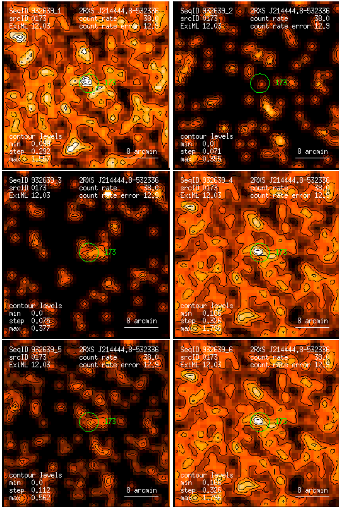
Figure 173: RASS 932639: detection 0173: band rate images, Gaussian filter: (1) PSPC channels 11 – 41, (2) 52 – 90, (3) 91 – 201, (4) 11 – 235, (5) 52 – 201, (6) 11 – 201. Broad band rates in counts/ks. Band rate contour levels in counts/ks/arcmin 2 .
