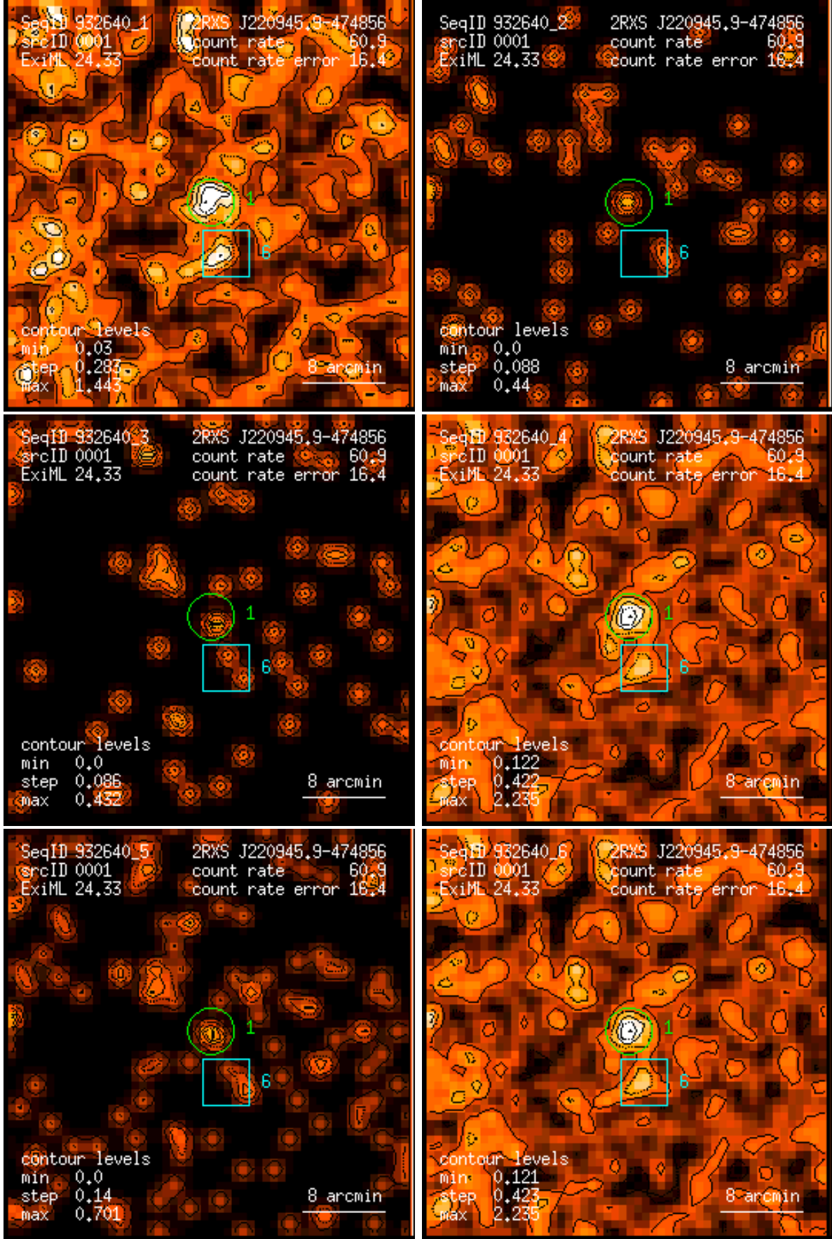
Figure 1: RASS 932640: detection 0001: band rate images, Gaussian filter: (1) PSPC channels 11 – 41, (2) 52 – 90, (3) 91 – 201, (4) 11 – 235, (5) 52 – 201, (6) 11 – 201. Broad band rates in counts/ks. Band rate contour levels in counts/ks/arcmin 2 .
