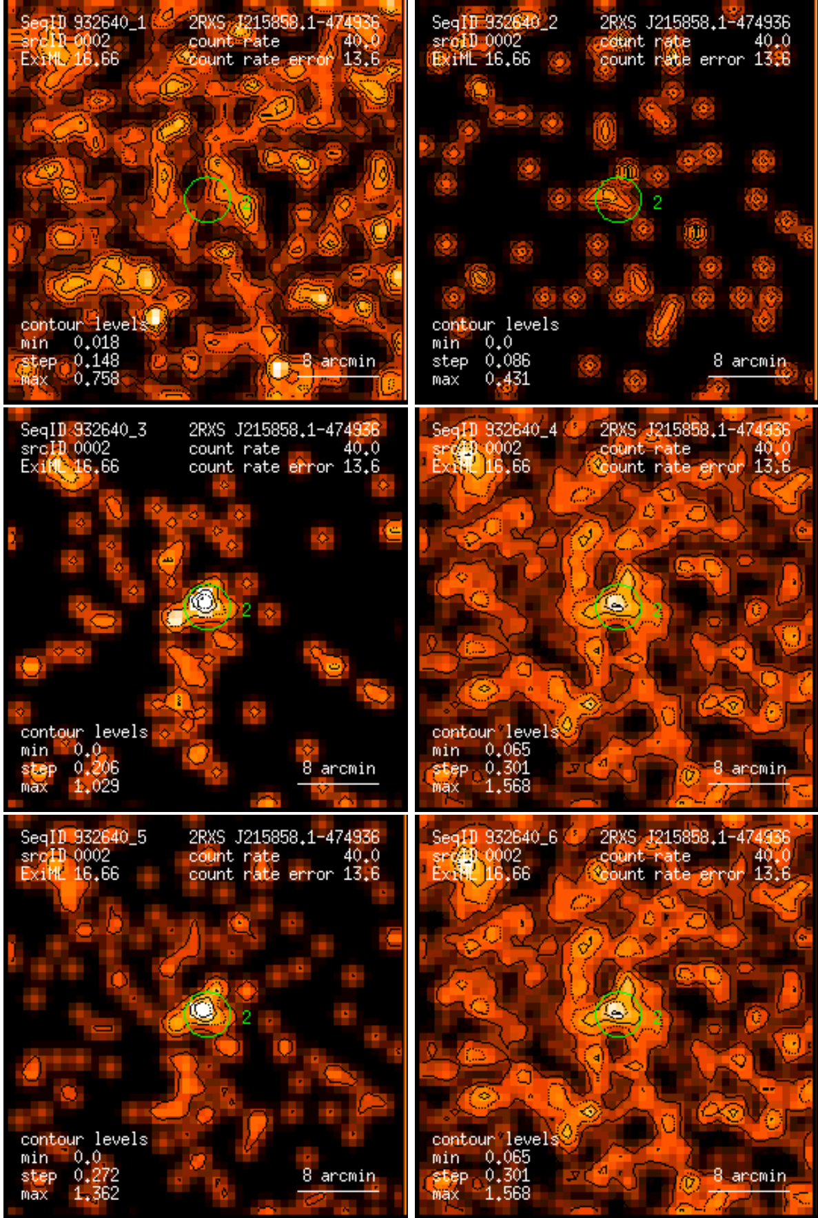
Figure 2: RASS 932640: detection 0002: band rate images, Gaussian filter: (1) PSPC channels 11 – 41, (2) 52 – 90, (3) 91 – 201, (4) 11 – 235, (5) 52 – 201, (6) 11 – 201. Broad band rates in counts/ks. Band rate contour levels in counts/ks/arcmin 2 .
