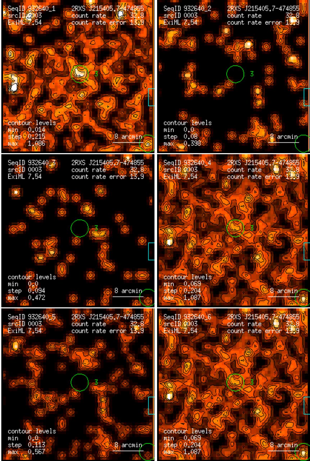
Figure 3: RASS 932640: detection 0003: band rate images, Gaussian filter: (1) PSPC channels 11 – 41, (2) 52 – 90, (3) 91 – 201, (4) 11 – 235, (5) 52 – 201, (6) 11 – 201. Broad band rates in counts/ks. Band rate contour levels in counts/ks/arcmin 2 .
