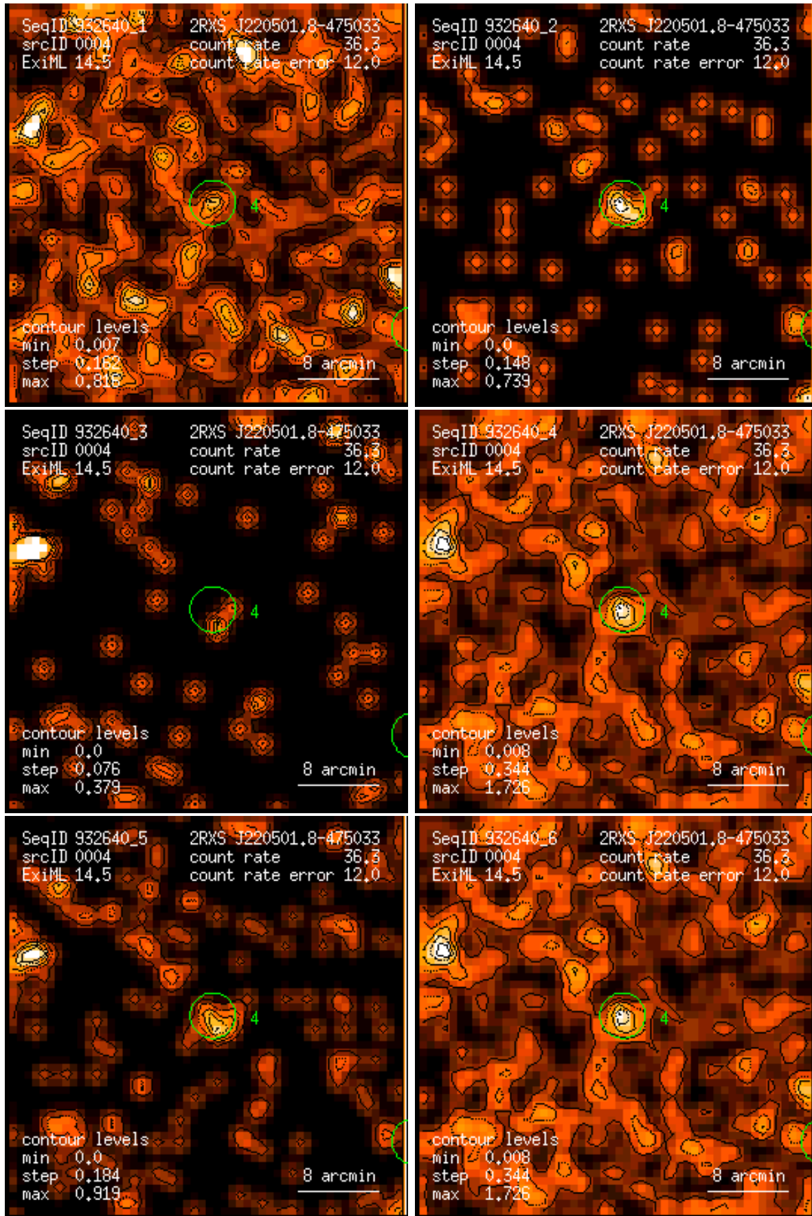
Figure 4: RASS 932640: detection 0004: band rate images, Gaussian filter: (1) PSPC channels 11 – 41, (2) 52 – 90, (3) 91 – 201, (4) 11 – 235, (5) 52 – 201, (6) 11 – 201. Broad band rates in counts/ks. Band rate contour levels in counts/ks/arcmin 2 .
