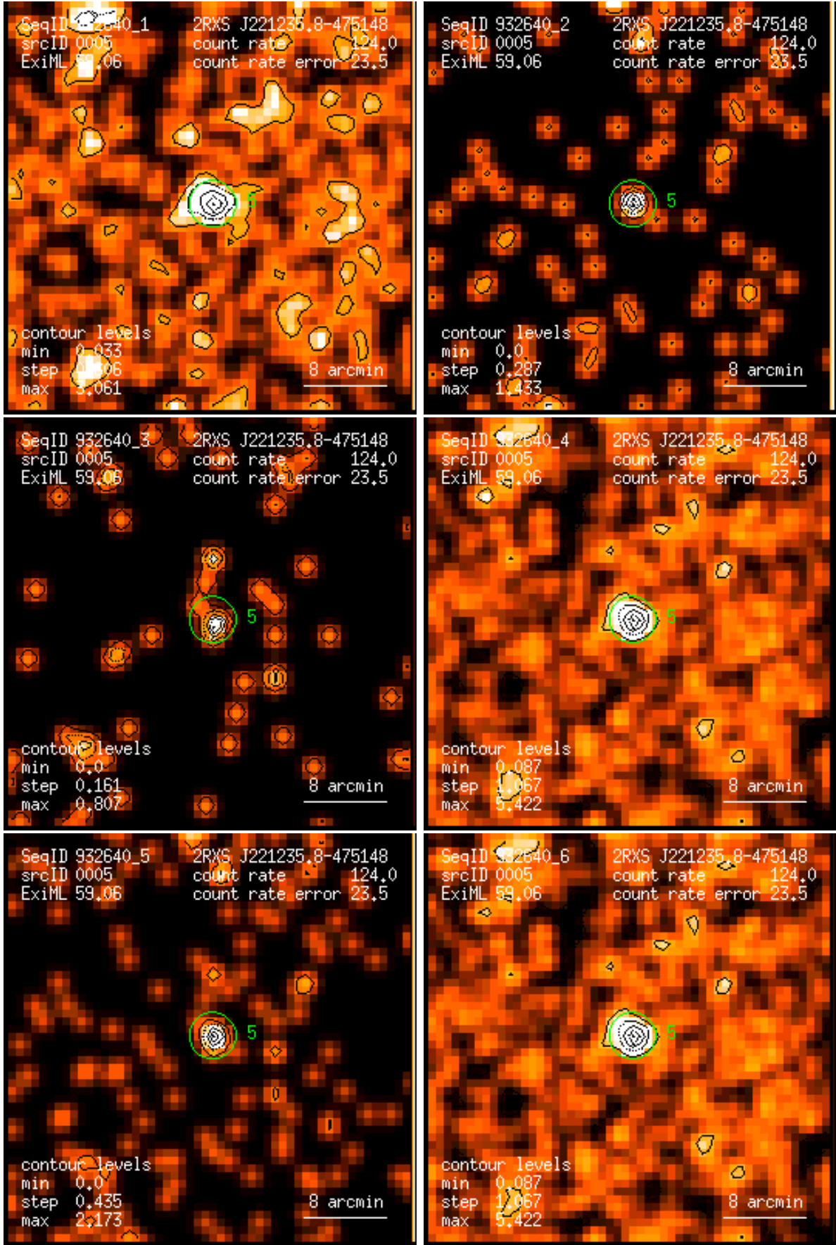
Figure 5: RASS 932640: detection 0005: band rate images, Gaussian filter: (1) PSPC channels 11 – 41, (2) 52 – 90, (3) 91 – 201, (4) 11 – 235, (5) 52 – 201, (6) 11 – 201. Broad band rates in counts/ks. Band rate contour levels in counts/ks/arcmin 2 .
