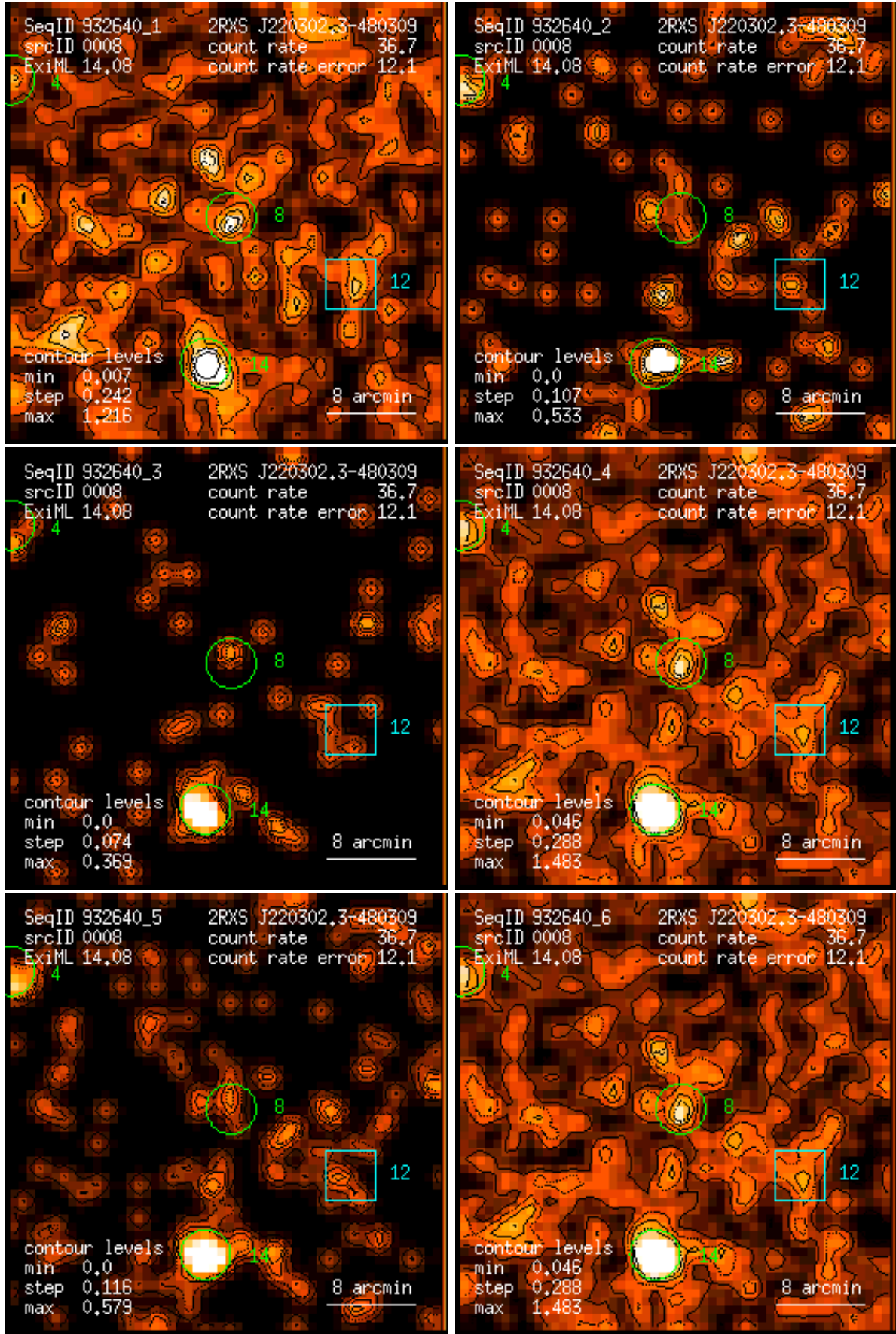
Figure 8: RASS 932640: detection 0008: band rate images, Gaussian filter: (1) PSPC channels 11 – 41, (2) 52 – 90, (3) 91 – 201, (4) 11 – 235, (5) 52 – 201, (6) 11 – 201. Broad band rates in counts/ks. Band rate contour levels in counts/ks/arcmin 2 .
