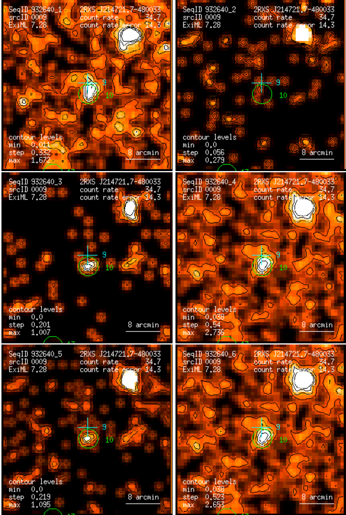
Figure 9: RASS 932640: detection 0009: band rate images, Gaussian filter: (1) PSPC channels 11 – 41, (2) 52 – 90, (3) 91 – 201, (4) 11 – 235, (5) 52 – 201, (6) 11 – 201. Broad band rates in counts/ks. Band rate contour levels in counts/ks/arcmin 2 .
