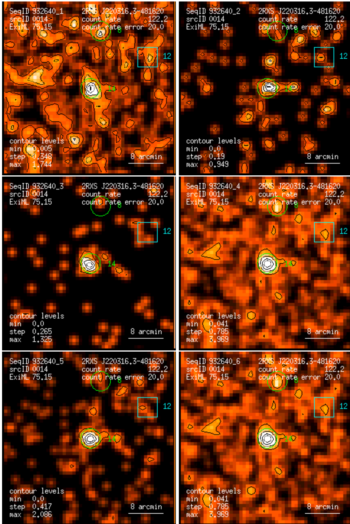
Figure 14: RASS 932640: detection 0014: band rate images, Gaussian filter: (1) PSPC channels 11 – 41, (2) 52 – 90, (3) 91 – 201, (4) 11 – 235, (5) 52 – 201, (6) 11 – 201. Broad band rates in counts/ks. Band rate contour levels in counts/ks/arcmin 2 .
