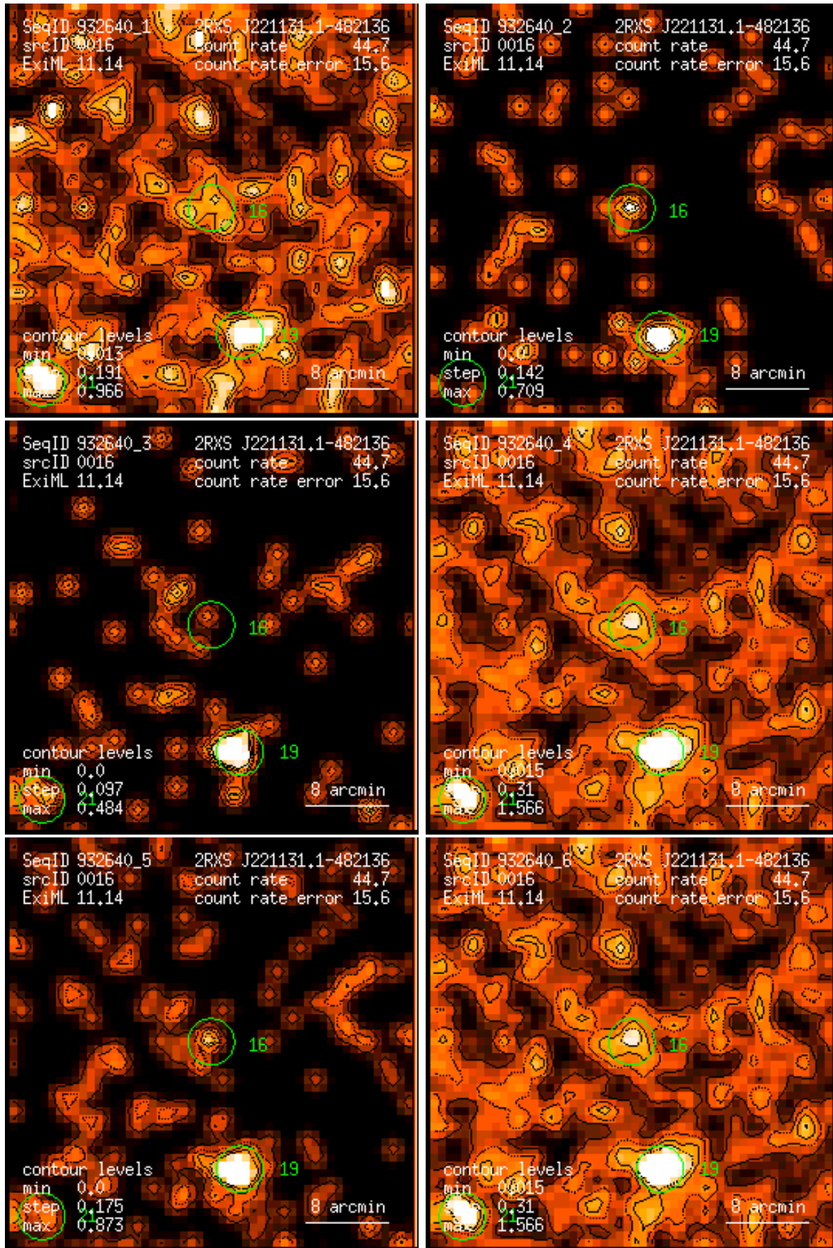
Figure 16: RASS 932640: detection 0016: band rate images, Gaussian filter: (1) PSPC channels 11 – 41, (2) 52 – 90, (3) 91 – 201, (4) 11 – 235, (5) 52 – 201, (6) 11 – 201. Broad band rates in counts/ks. Band rate contour levels in counts/ks/arcmin 2 .
