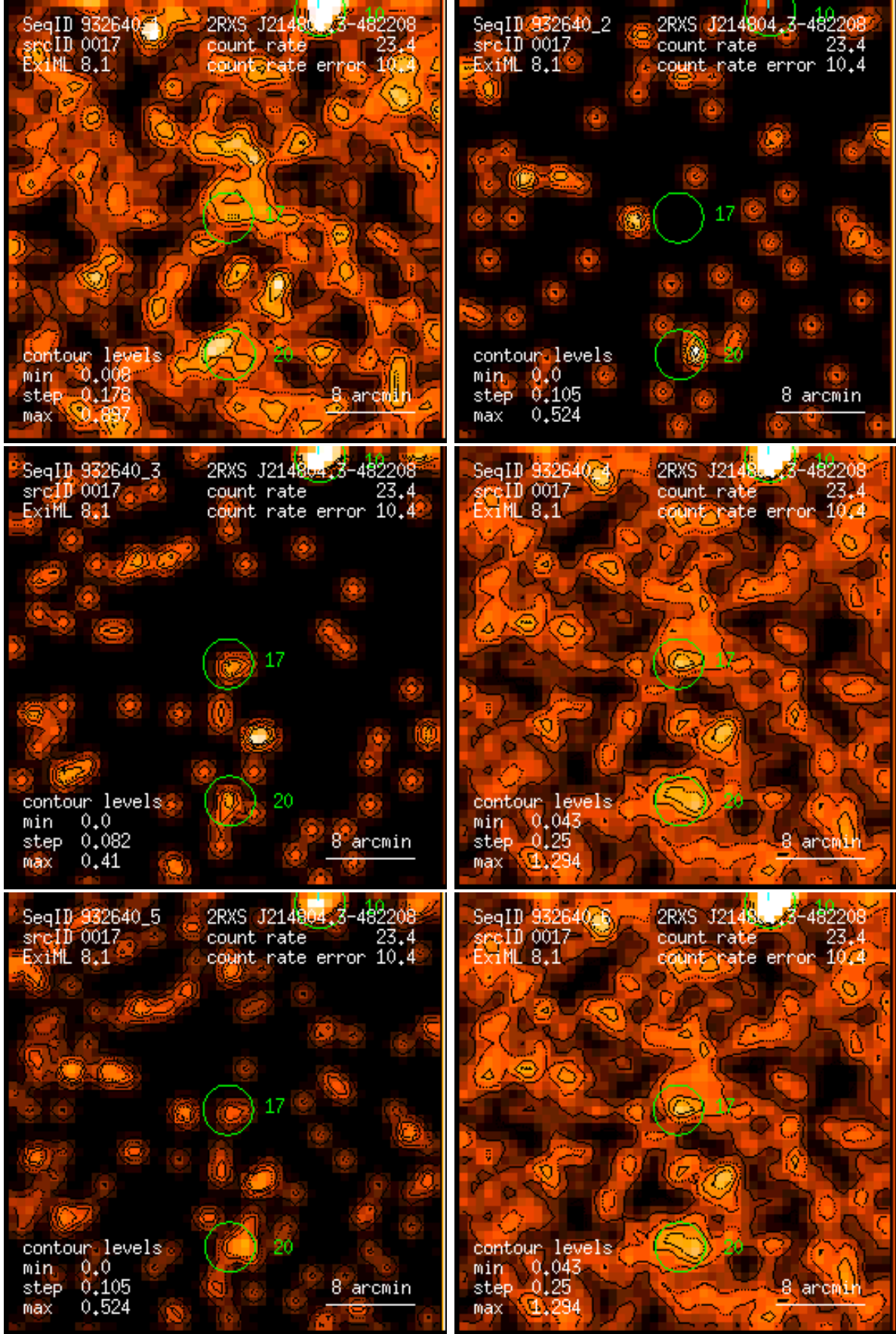
Figure 17: RASS 932640: detection 0017: band rate images, Gaussian filter: (1) PSPC channels 11 – 41, (2) 52 – 90, (3) 91 – 201, (4) 11 – 235, (5) 52 – 201, (6) 11 – 201. Broad band rates in counts/ks. Band rate contour levels in counts/ks/arcmin 2 .
