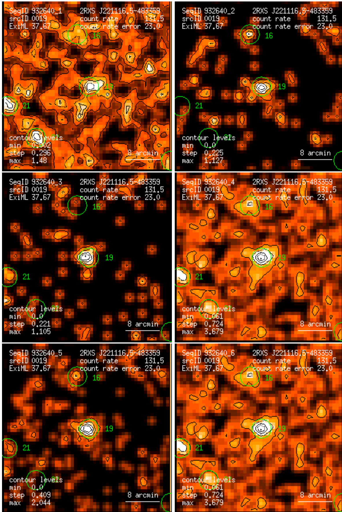
Figure 19: RASS 932640: detection 0019: band rate images, Gaussian filter: (1) PSPC channels 11 – 41, (2) 52 – 90, (3) 91 – 201, (4) 11 – 235, (5) 52 – 201, (6) 11 – 201. Broad band rates in counts/ks. Band rate contour levels in counts/ks/arcmin 2 .
