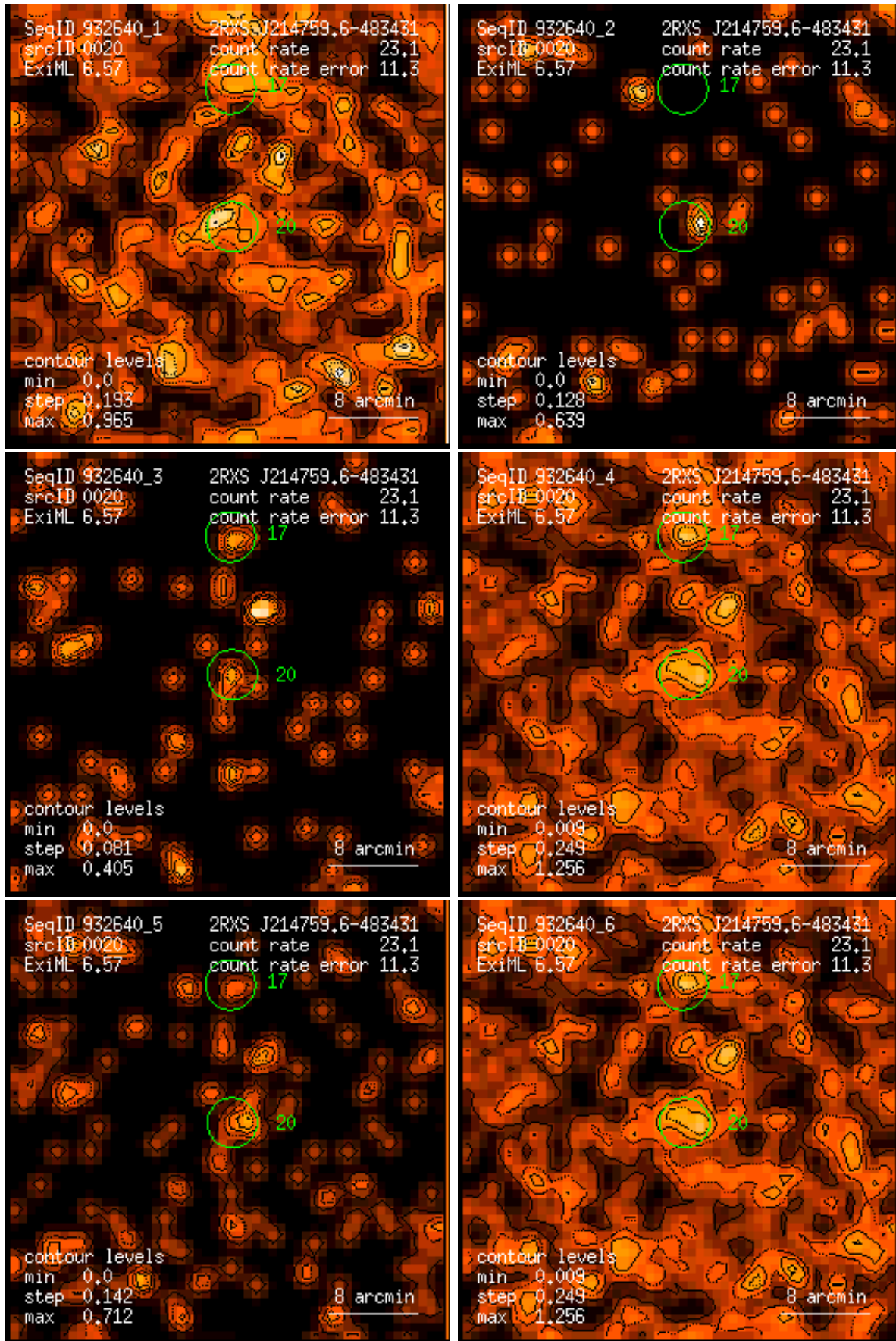
Figure 20: RASS 932640: detection 0020: band rate images, Gaussian filter: (1) PSPC channels 11 – 41, (2) 52 – 90, (3) 91 – 201, (4) 11 – 235, (5) 52 – 201, (6) 11 – 201. Broad band rates in counts/ks. Band rate contour levels in counts/ks/arcmin 2 .
