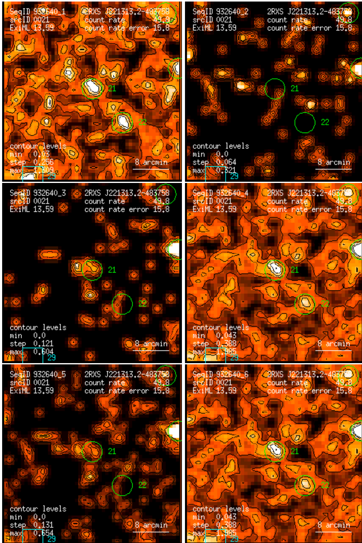
Figure 21: RASS 932640: detection 0021: band rate images, Gaussian filter: (1) PSPC channels 11 – 41, (2) 52 – 90, (3) 91 – 201, (4) 11 – 235, (5) 52 – 201, (6) 11 – 201. Broad band rates in counts/ks. Band rate contour levels in counts/ks/arcmin 2 .
