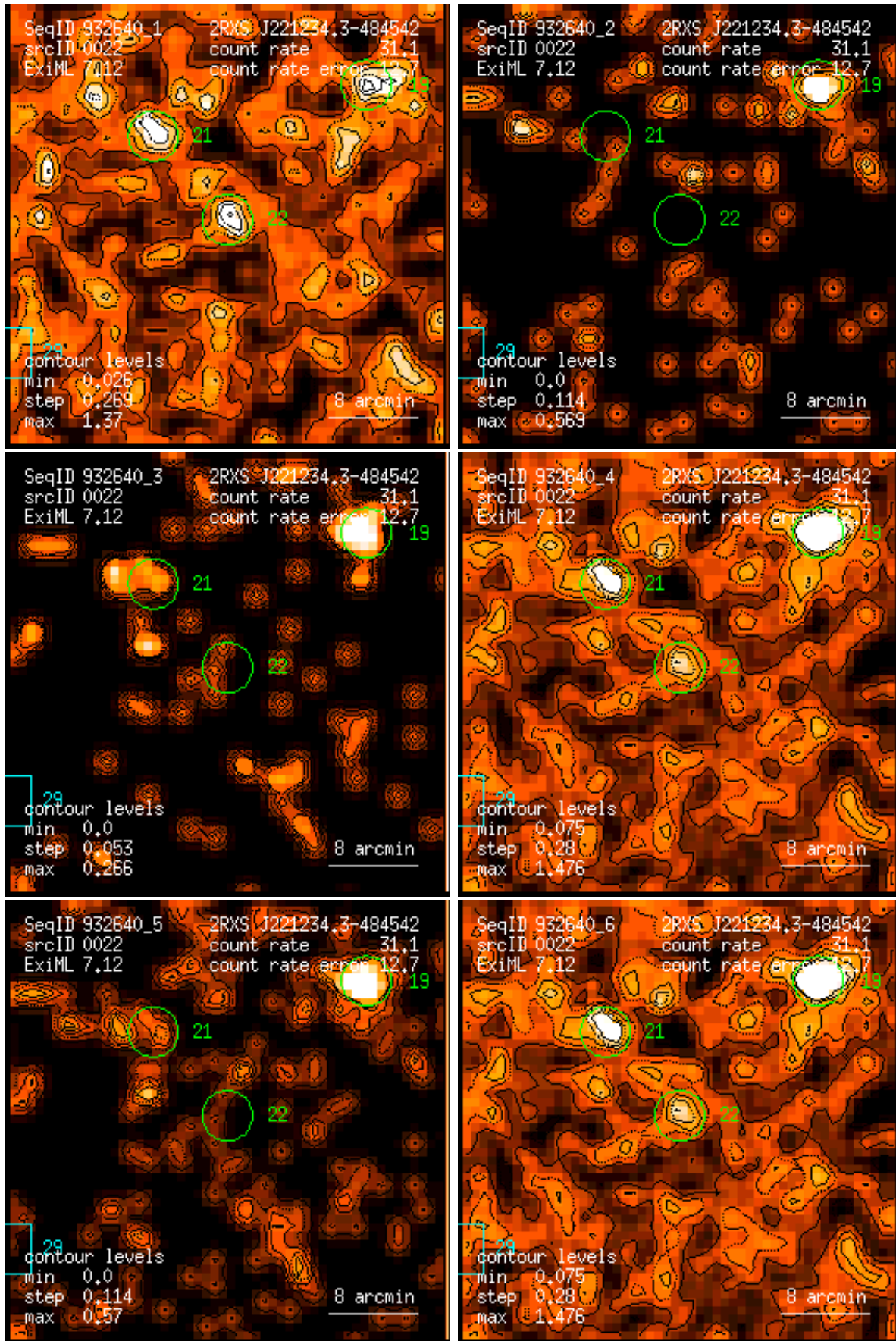
Figure 22: RASS 932640: detection 0022: band rate images, Gaussian filter: (1) PSPC channels 11 – 41, (2) 52 – 90, (3) 91 – 201, (4) 11 – 235, (5) 52 – 201, (6) 11 – 201. Broad band rates in counts/ks. Band rate contour levels in counts/ks/arcmin 2 .
