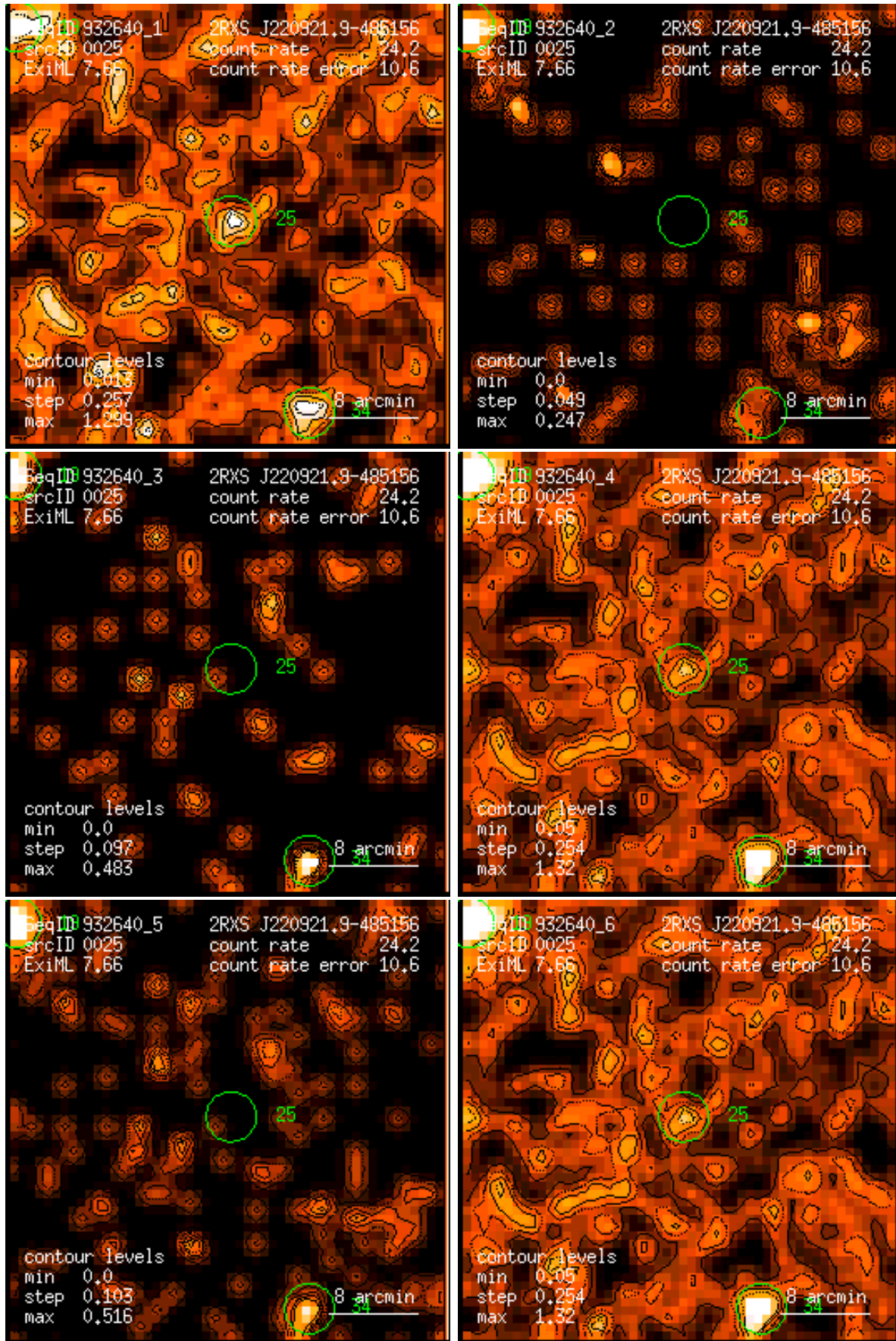
Figure 25: RASS 932640: detection 0025: band rate images, Gaussian filter: (1) PSPC channels 11 – 41, (2) 52 – 90, (3) 91 – 201, (4) 11 – 235, (5) 52 – 201, (6) 11 – 201. Broad band rates in counts/ks. Band rate contour levels in counts/ks/arcmin 2 .
