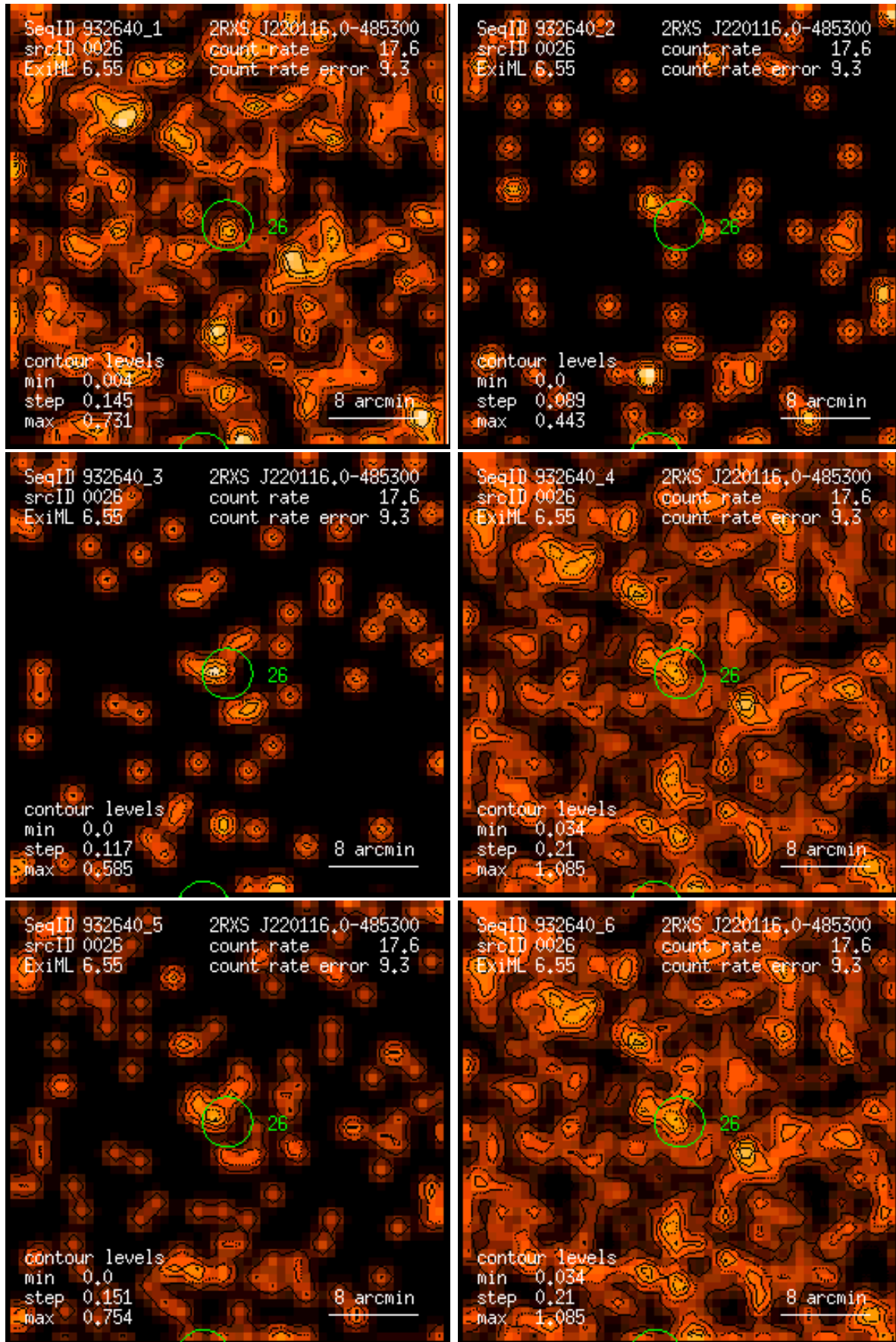
Figure 26: RASS 932640: detection 0026: band rate images, Gaussian filter: (1) PSPC channels 11 – 41, (2) 52 – 90, (3) 91 – 201, (4) 11 – 235, (5) 52 – 201, (6) 11 – 201. Broad band rates in counts/ks. Band rate contour levels in counts/ks/arcmin 2 .
