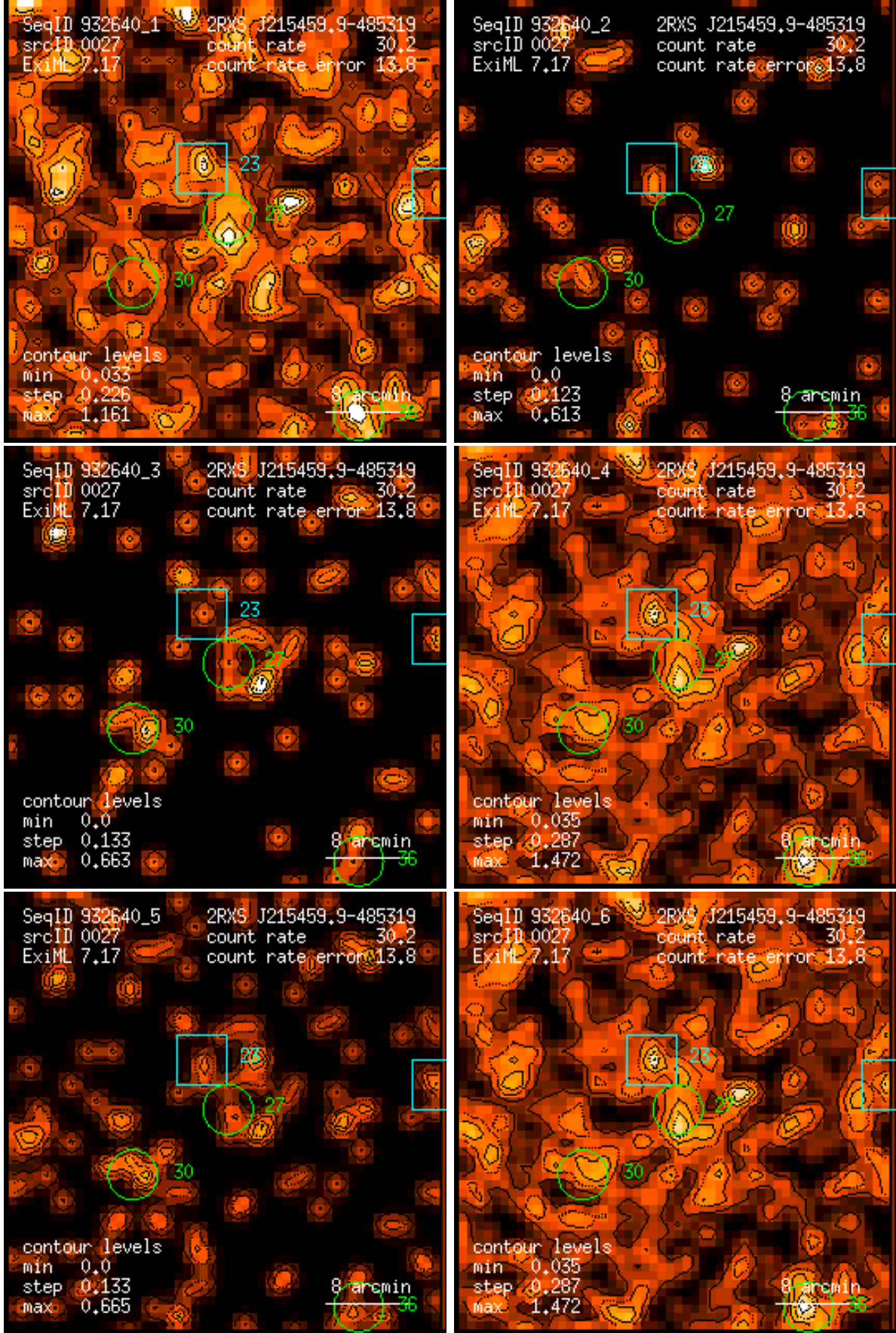
Figure 27: RASS 932640: detection 0027: band rate images, Gaussian filter: (1) PSPC channels 11 – 41, (2) 52 – 90, (3) 91 – 201, (4) 11 – 235, (5) 52 – 201, (6) 11 – 201. Broad band rates in counts/ks. Band rate contour levels in counts/ks/arcmin 2 .
