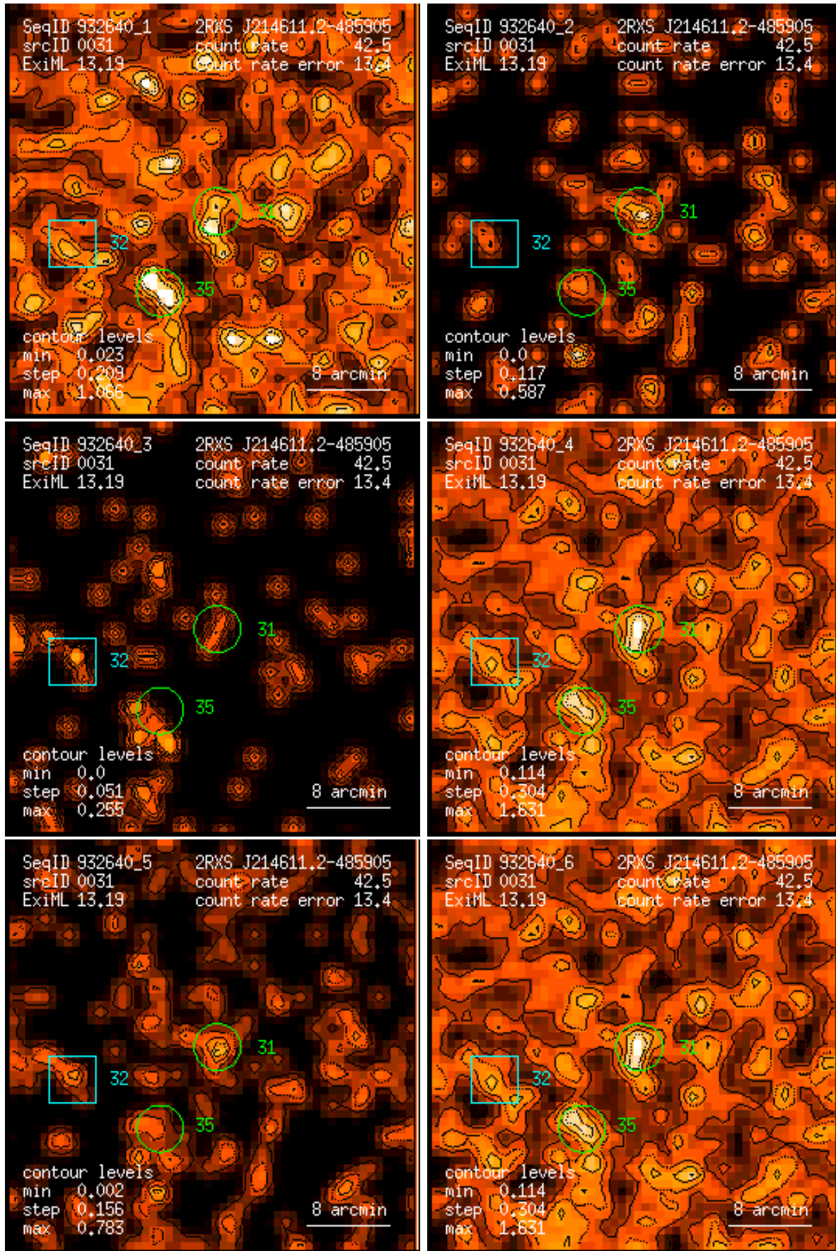
Figure 31: RASS 932640: detection 0031: band rate images, Gaussian filter: (1) PSPC channels 11 – 41, (2) 52 – 90, (3) 91 – 201, (4) 11 – 235, (5) 52 – 201, (6) 11 – 201. Broad band rates in counts/ks. Band rate contour levels in counts/ks/arcmin 2 .
