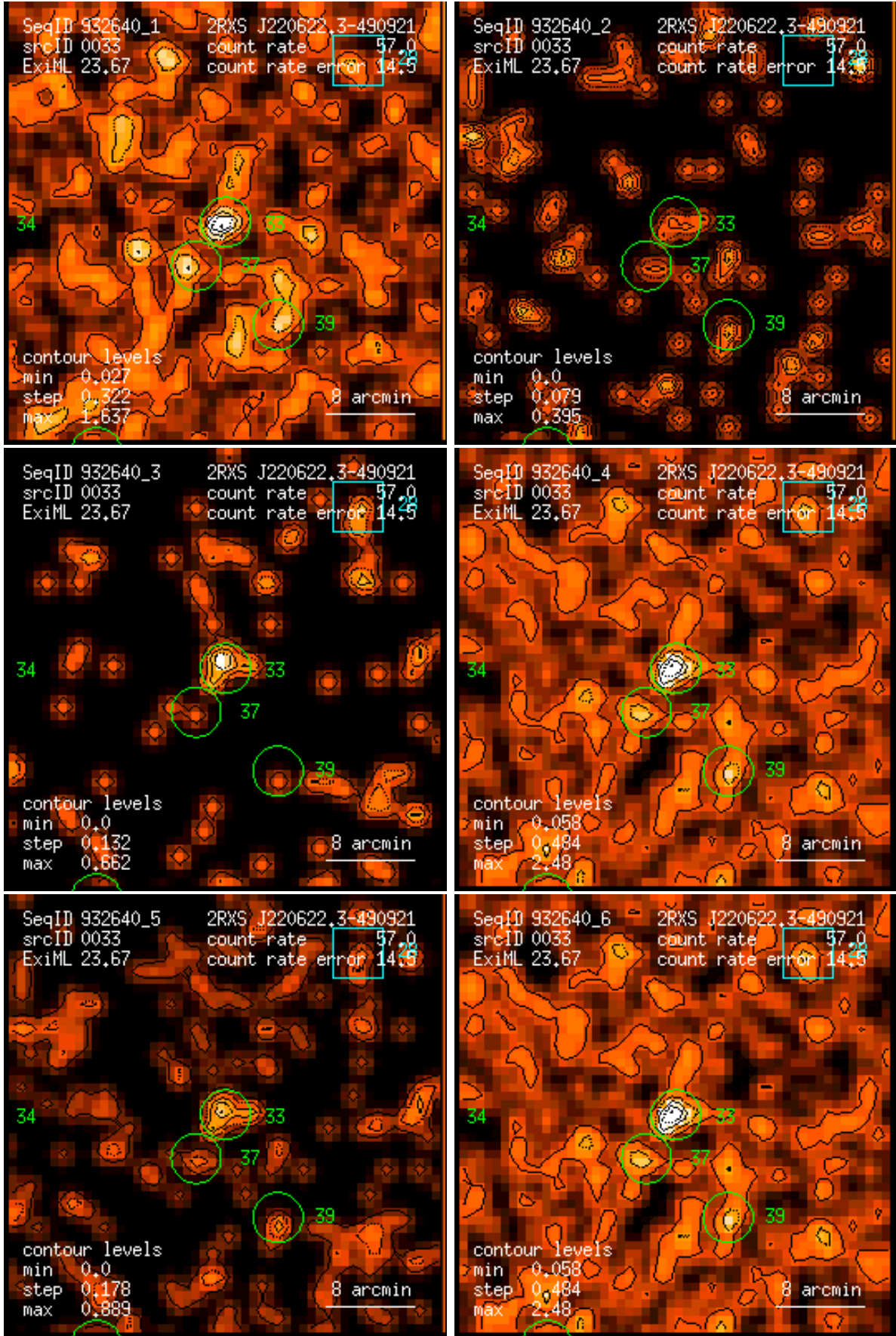
Figure 33: RASS 932640: detection 0033: band rate images, Gaussian filter: (1) PSPC channels 11 – 41, (2) 52 – 90, (3) 91 – 201, (4) 11 – 235, (5) 52 – 201, (6) 11 – 201. Broad band rates in counts/ks. Band rate contour levels in counts/ks/arcmin 2 .
