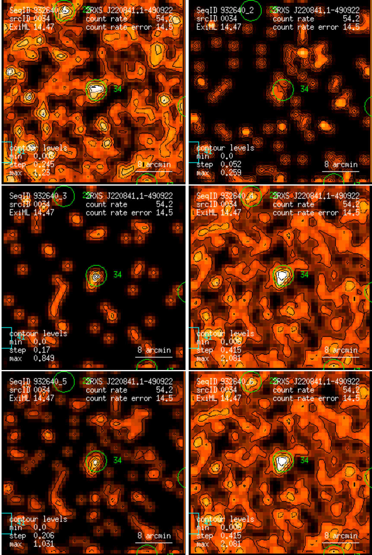
Figure 34: RASS 932640: detection 0034: band rate images, Gaussian filter: (1) PSPC channels 11 – 41, (2) 52 – 90, (3) 91 – 201, (4) 11 – 235, (5) 52 – 201, (6) 11 – 201. Broad band rates in counts/ks. Band rate contour levels in counts/ks/arcmin 2 .
