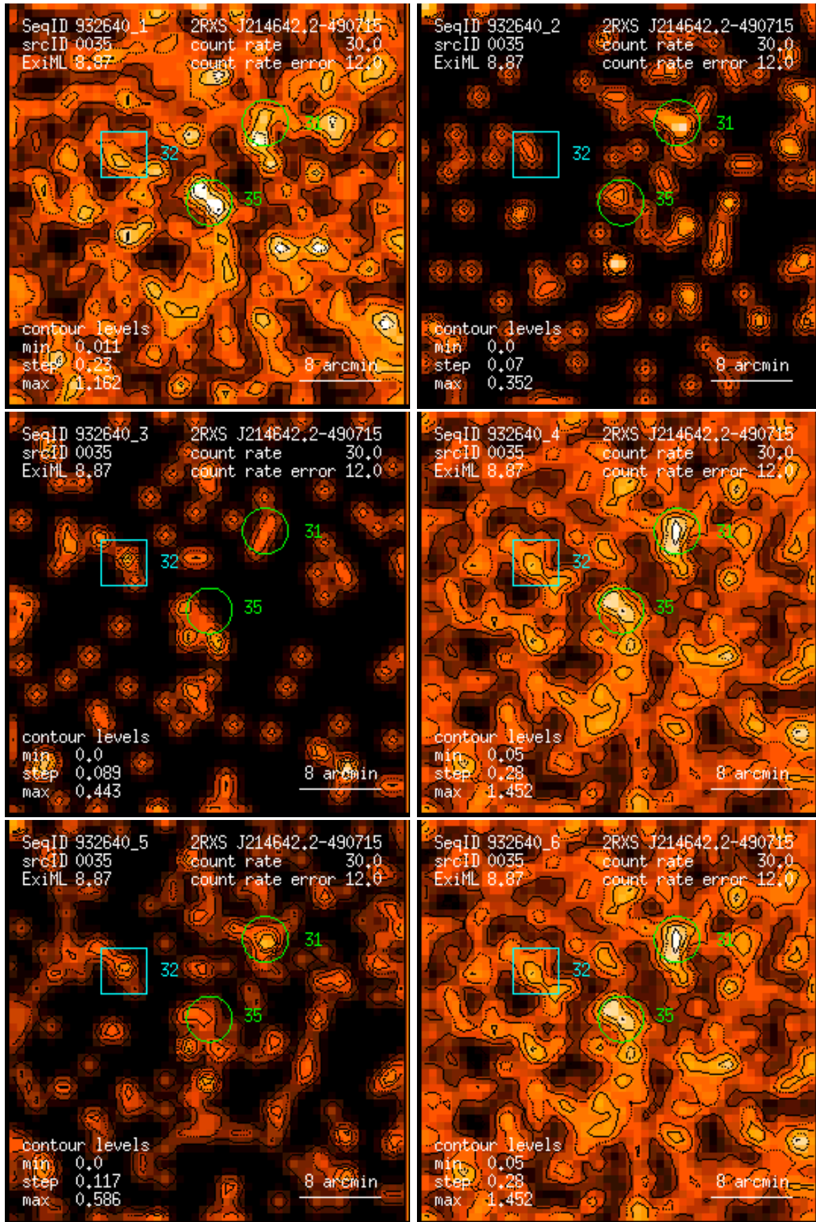
Figure 35: RASS 932640: detection 0035: band rate images, Gaussian filter: (1) PSPC channels 11 – 41, (2) 52 – 90, (3) 91 – 201, (4) 11 – 235, (5) 52 – 201, (6) 11 – 201. Broad band rates in counts/ks. Band rate contour levels in counts/ks/arcmin 2 .
