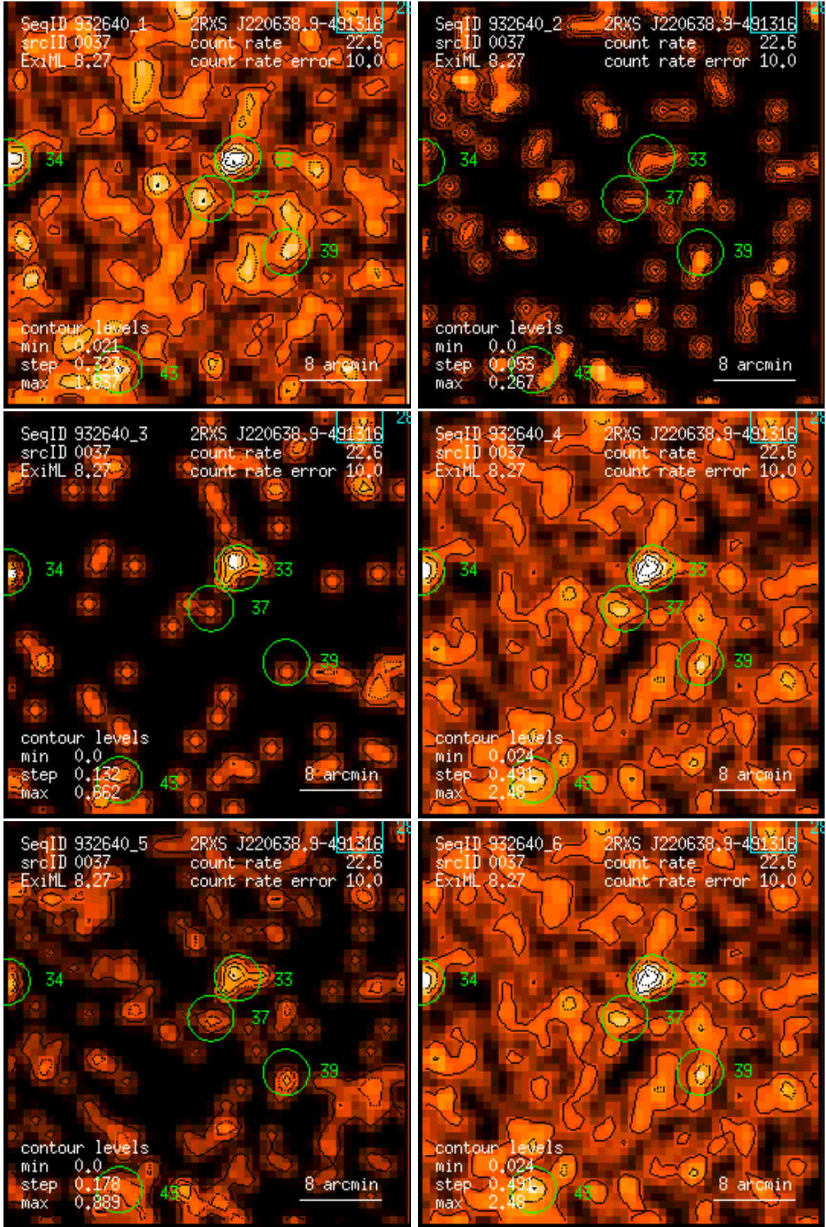
Figure 37: RASS 932640: detection 0037: band rate images, Gaussian filter: (1) PSPC channels 11 – 41, (2) 52 – 90, (3) 91 – 201, (4) 11 – 235, (5) 52 – 201, (6) 11 – 201. Broad band rates in counts/ks. Band rate contour levels in counts/ks/arcmin 2 .
