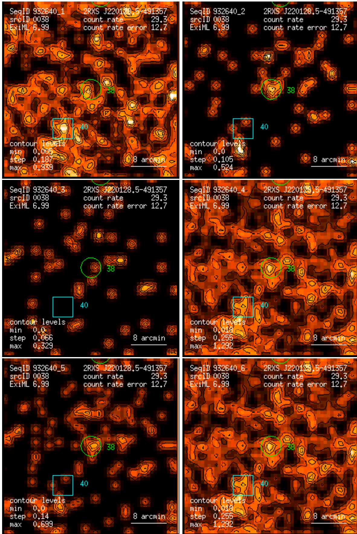
Figure 38: RASS 932640: detection 0038: band rate images, Gaussian filter: (1) PSPC channels 11 – 41, (2) 52 – 90, (3) 91 – 201, (4) 11 – 235, (5) 52 – 201, (6) 11 – 201. Broad band rates in counts/ks. Band rate contour levels in counts/ks/arcmin 2 .
