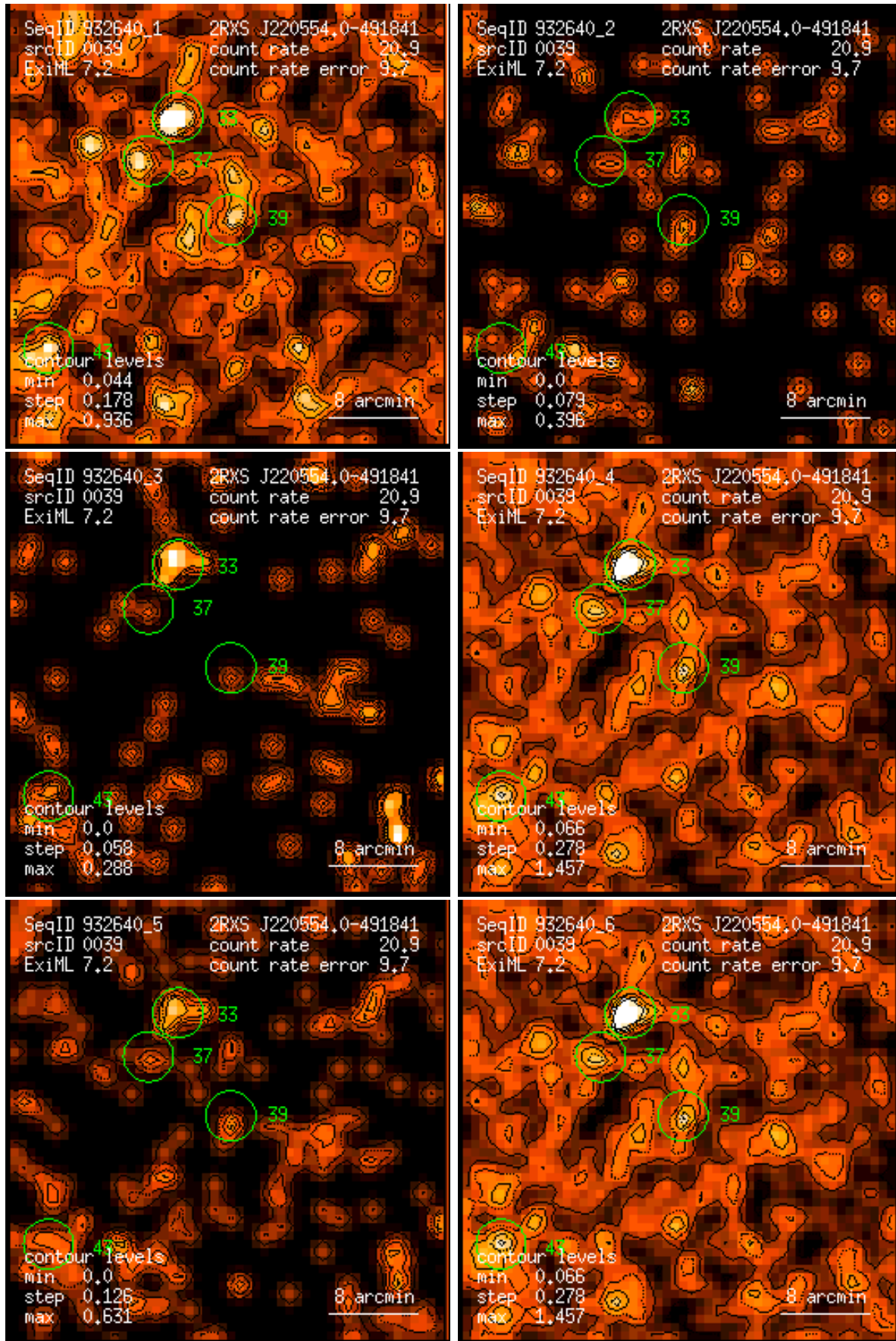
Figure 39: RASS 932640: detection 0039: band rate images, Gaussian filter: (1) PSPC channels 11 – 41, (2) 52 – 90, (3) 91 – 201, (4) 11 – 235, (5) 52 – 201, (6) 11 – 201. Broad band rates in counts/ks. Band rate contour levels in counts/ks/arcmin 2 .
