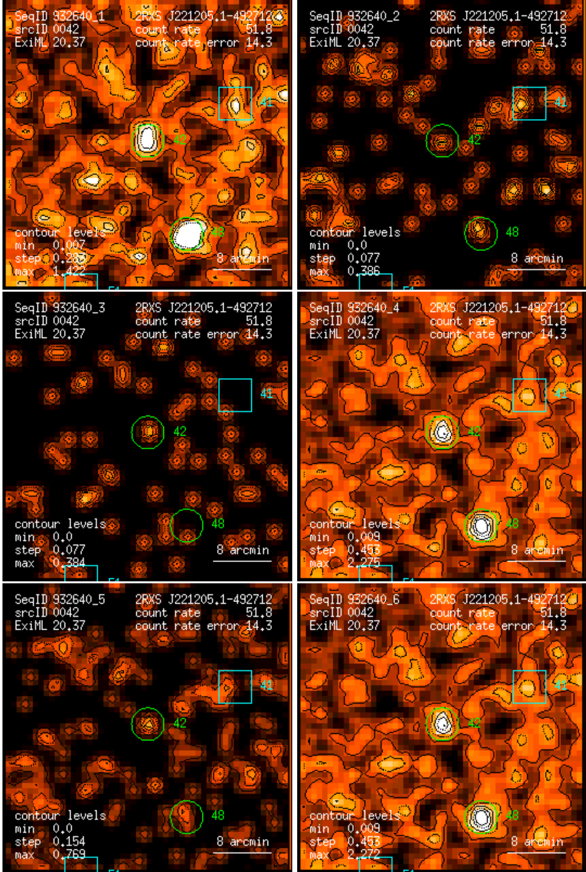
Figure 42: RASS 932640: detection 0042: band rate images, Gaussian filter: (1) PSPC channels 11 – 41, (2) 52 – 90, (3) 91 – 201, (4) 11 – 235, (5) 52 – 201, (6) 11 – 201. Broad band rates in counts/ks. Band rate contour levels in counts/ks/arcmin 2 .
