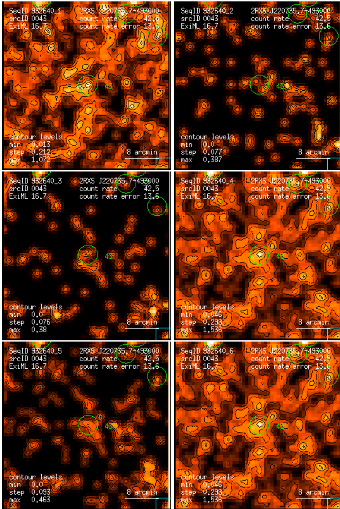
Figure 43: RASS 932640: detection 0043: band rate images, Gaussian filter: (1) PSPC channels 11 – 41, (2) 52 – 90, (3) 91 – 201, (4) 11 – 235, (5) 52 – 201, (6) 11 – 201. Broad band rates in counts/ks. Band rate contour levels in counts/ks/arcmin 2 .
