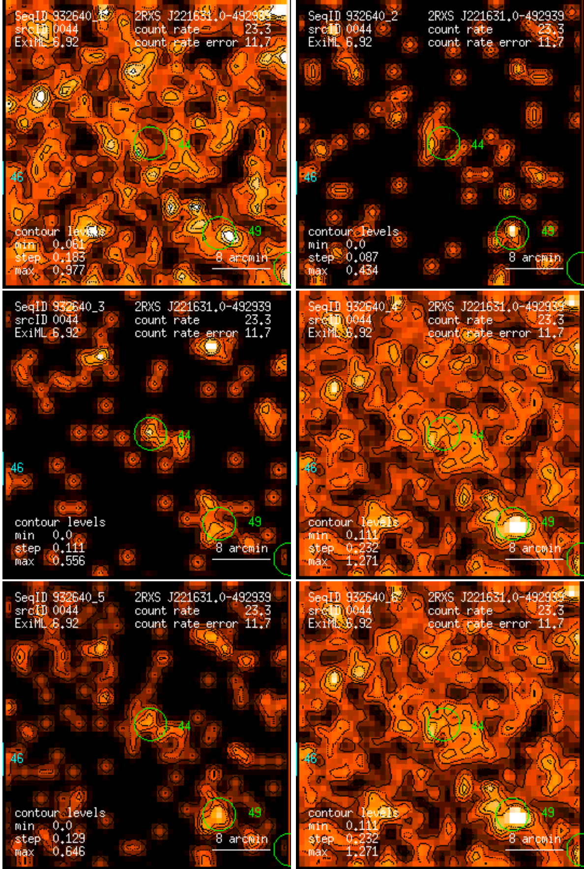
Figure 44: RASS 932640: detection 0044: band rate images, Gaussian filter: (1) PSPC channels 11 – 41, (2) 52 – 90, (3) 91 – 201, (4) 11 – 235, (5) 52 – 201, (6) 11 – 201. Broad band rates in counts/ks. Band rate contour levels in counts/ks/arcmin 2 .
