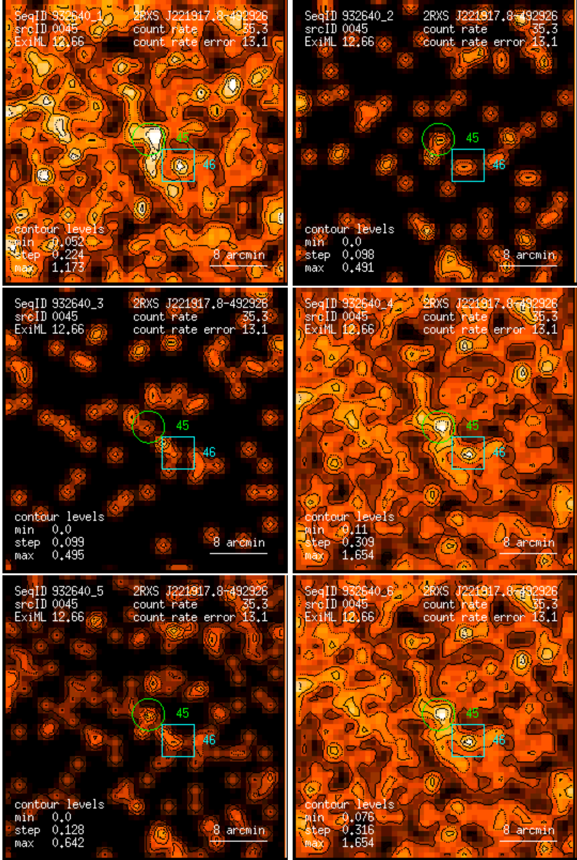
Figure 45: RASS 932640: detection 0045: band rate images, Gaussian filter: (1) PSPC channels 11 – 41, (2) 52 – 90, (3) 91 – 201, (4) 11 – 235, (5) 52 – 201, (6) 11 – 201. Broad band rates in counts/ks. Band rate contour levels in counts/ks/arcmin 2 .
