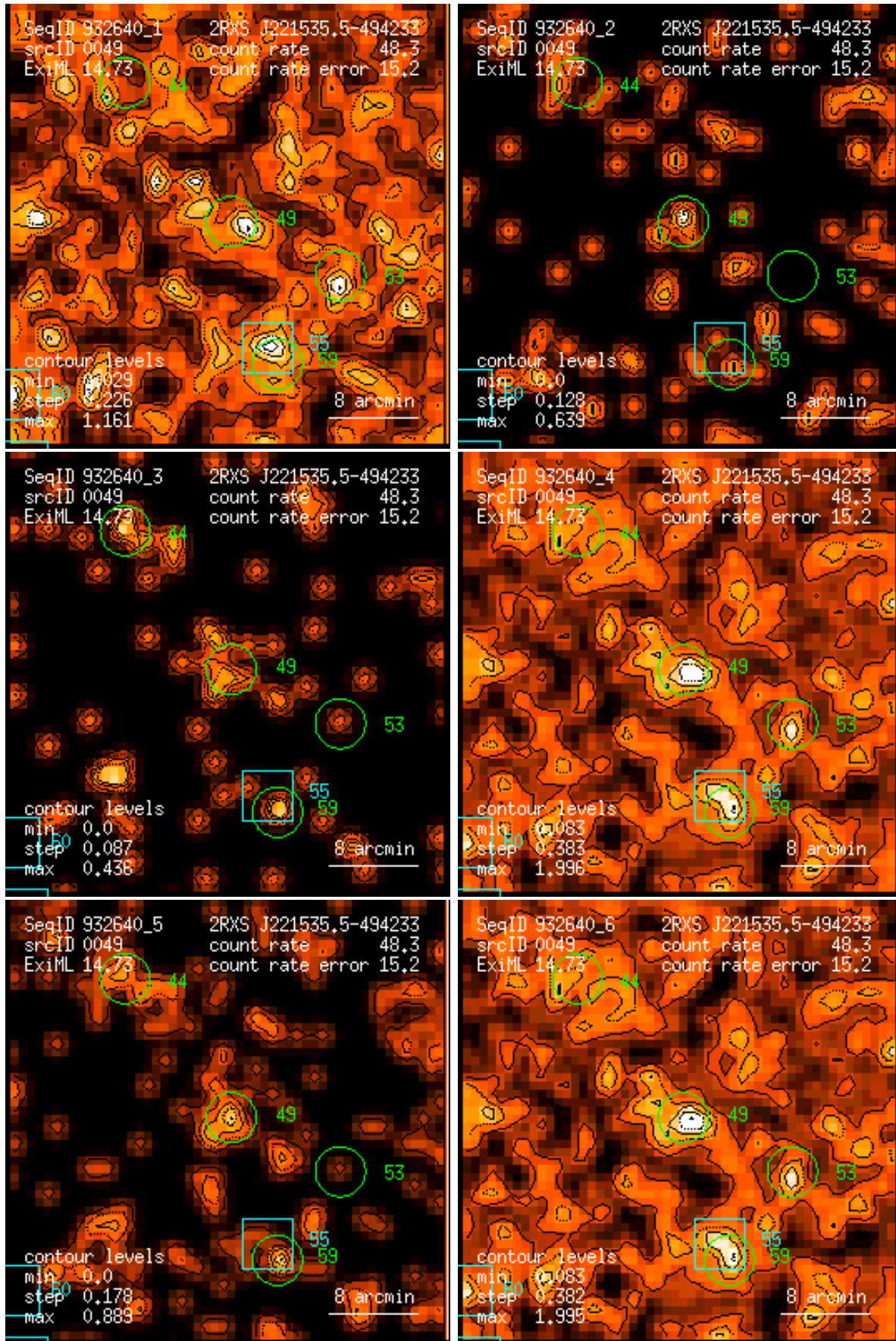
Figure 49: RASS 932640: detection 0049: band rate images, Gaussian filter: (1) PSPC channels 11 – 41, (2) 52 – 90, (3) 91 – 201, (4) 11 – 235, (5) 52 – 201, (6) 11 – 201. Broad band rates in counts/ks. Band rate contour levels in counts/ks/arcmin 2 .
