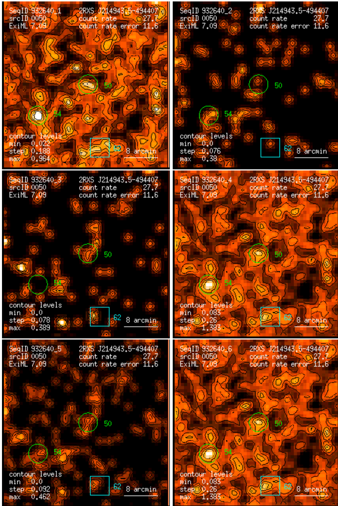
Figure 50: RASS 932640: detection 0050: band rate images, Gaussian filter: (1) PSPC channels 11 – 41, (2) 52 – 90, (3) 91 – 201, (4) 11 – 235, (5) 52 – 201, (6) 11 – 201. Broad band rates in counts/ks. Band rate contour levels in counts/ks/arcmin 2 .
