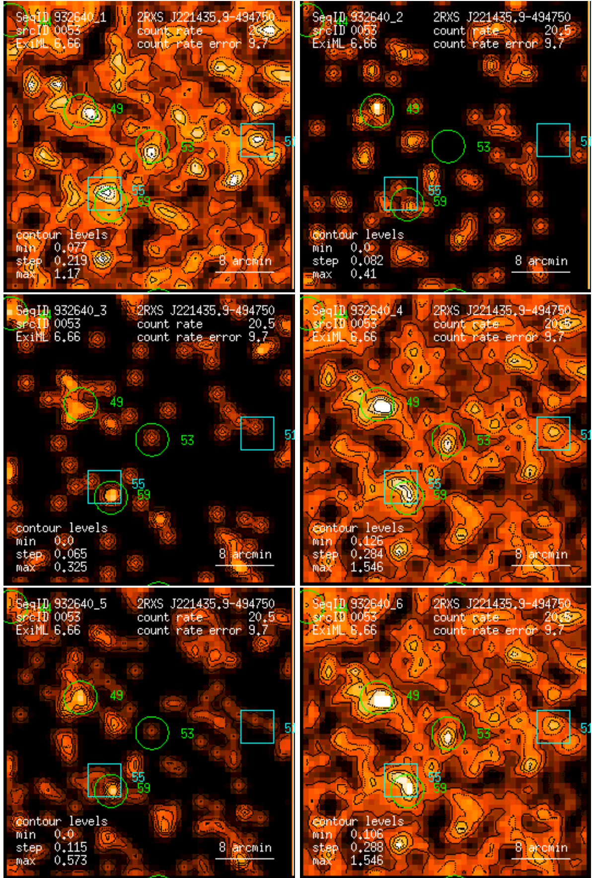
Figure 53: RASS 932640: detection 0053: band rate images, Gaussian filter: (1) PSPC channels 11 – 41, (2) 52 – 90, (3) 91 – 201, (4) 11 – 235, (5) 52 – 201, (6) 11 – 201. Broad band rates in counts/ks. Band rate contour levels in counts/ks/arcmin 2 .
