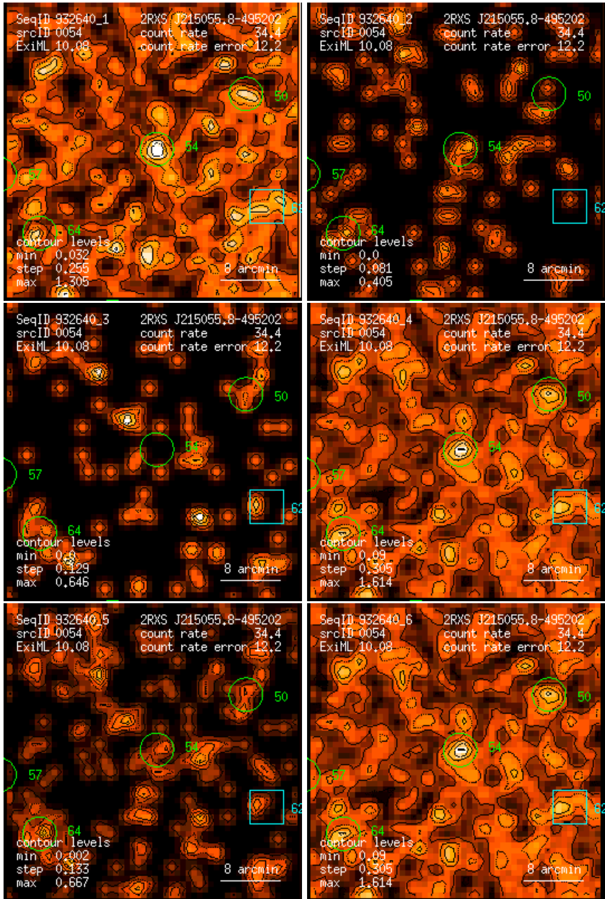
Figure 54: RASS 932640: detection 0054: band rate images, Gaussian filter: (1) PSPC channels 11 – 41, (2) 52 – 90, (3) 91 – 201, (4) 11 – 235, (5) 52 – 201, (6) 11 – 201. Broad band rates in counts/ks. Band rate contour levels in counts/ks/arcmin 2 .
