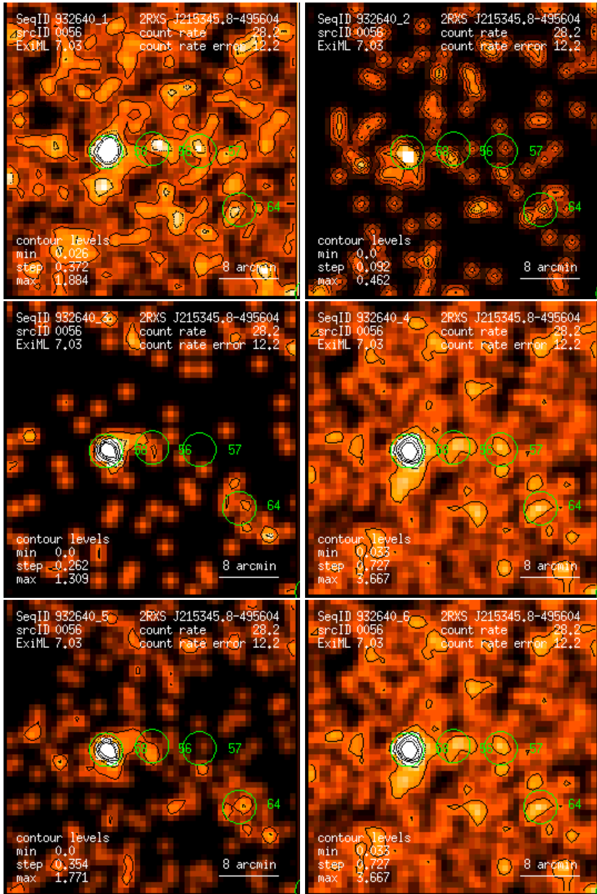
Figure 56: RASS 932640: detection 0056: band rate images, Gaussian filter: (1) PSPC channels 11 – 41, (2) 52 – 90, (3) 91 – 201, (4) 11 – 235, (5) 52 – 201, (6) 11 – 201. Broad band rates in counts/ks. Band rate contour levels in counts/ks/arcmin 2 .
