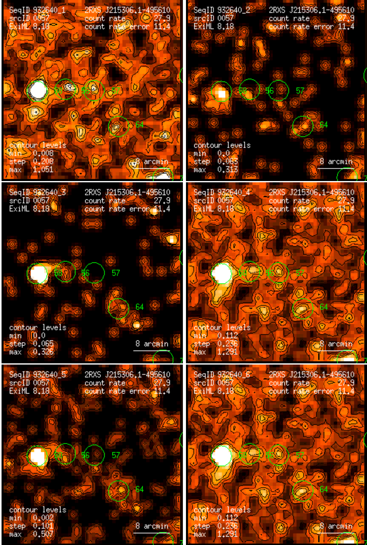
Figure 57: RASS 932640: detection 0057: band rate images, Gaussian filter: (1) PSPC channels 11 – 41, (2) 52 – 90, (3) 91 – 201, (4) 11 – 235, (5) 52 – 201, (6) 11 – 201. Broad band rates in counts/ks. Band rate contour levels in counts/ks/arcmin 2 .
