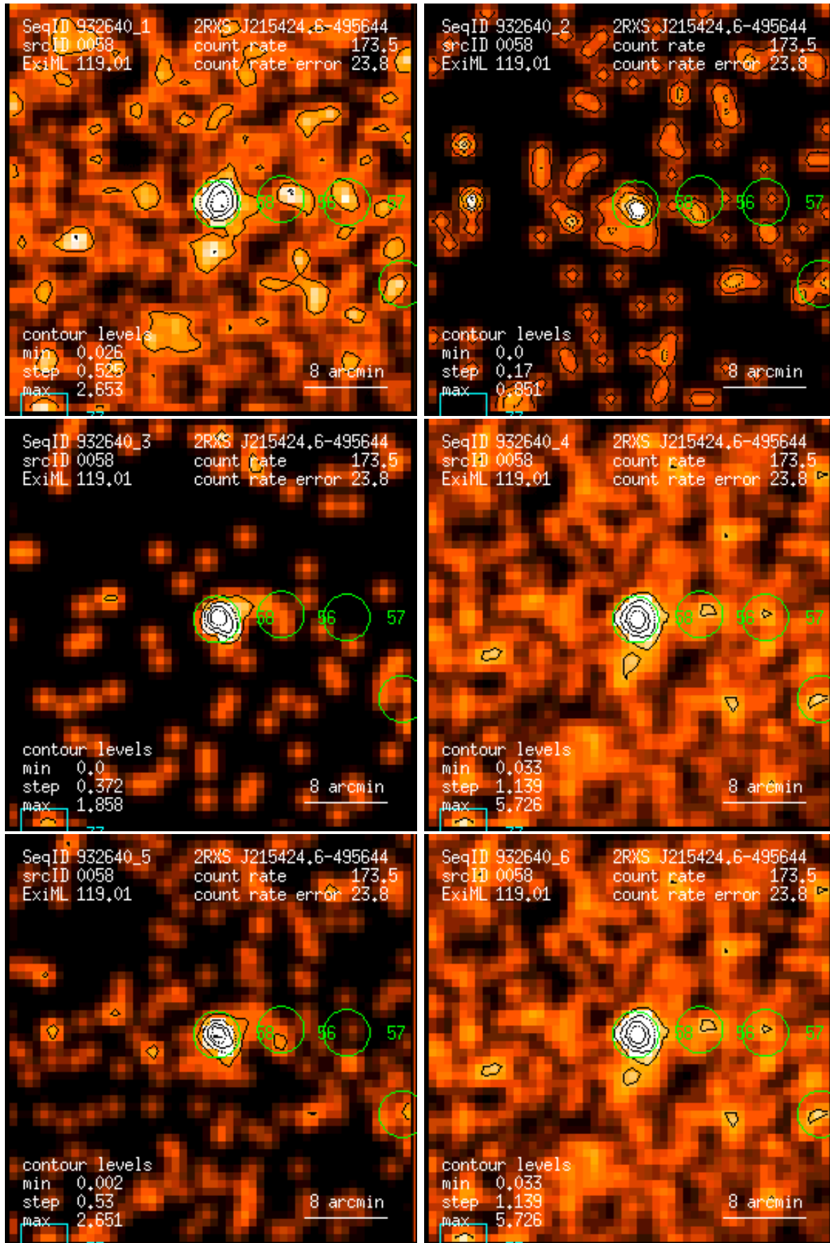
Figure 58: RASS 932640: detection 0058: band rate images, Gaussian filter: (1) PSPC channels 11 – 41, (2) 52 – 90, (3) 91 – 201, (4) 11 – 235, (5) 52 – 201, (6) 11 – 201. Broad band rates in counts/ks. Band rate contour levels in counts/ks/arcmin 2 .
