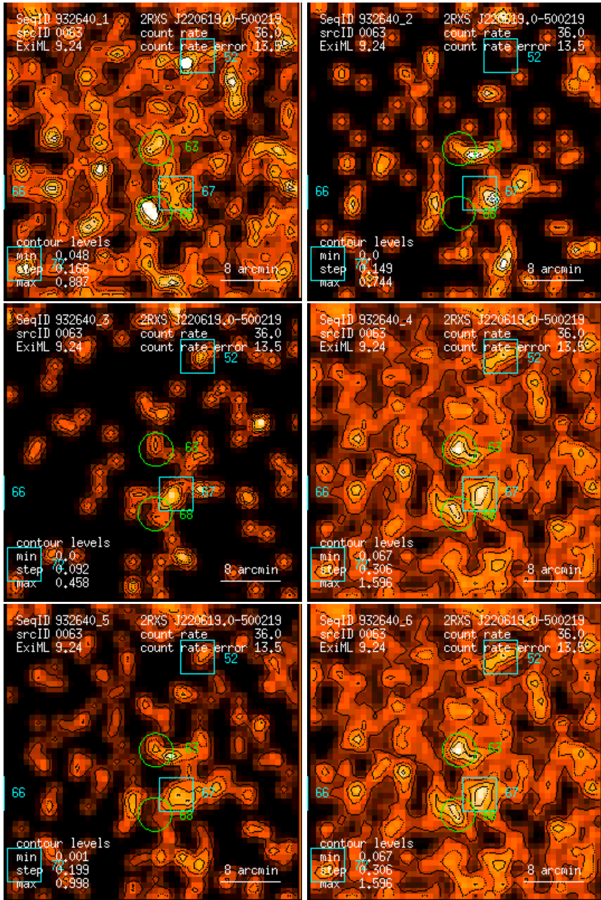
Figure 63: RASS 932640: detection 0063: band rate images, Gaussian filter: (1) PSPC channels 11 – 41, (2) 52 – 90, (3) 91 – 201, (4) 11 – 235, (5) 52 – 201, (6) 11 – 201. Broad band rates in counts/ks. Band rate contour levels in counts/ks/arcmin 2 .
