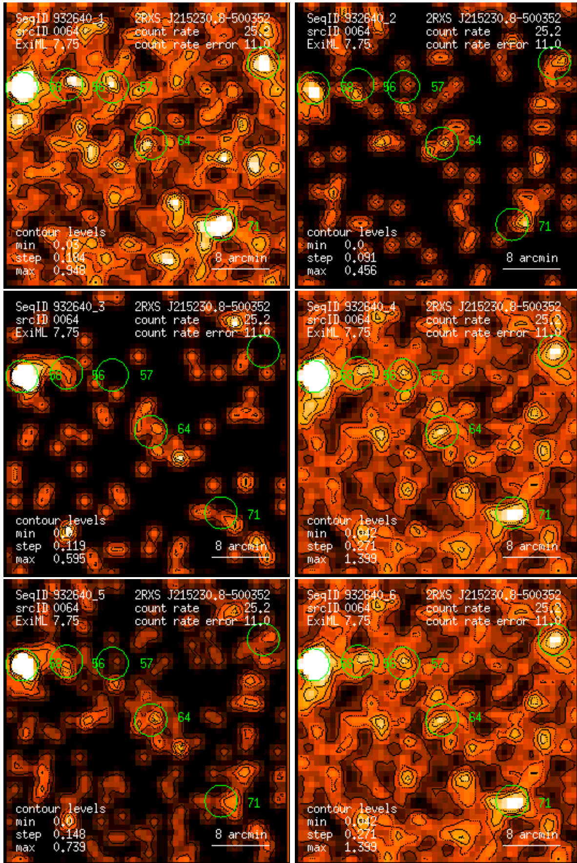
Figure 64: RASS 932640: detection 0064: band rate images, Gaussian filter: (1) PSPC channels 11 – 41, (2) 52 – 90, (3) 91 – 201, (4) 11 – 235, (5) 52 – 201, (6) 11 – 201. Broad band rates in counts/ks. Band rate contour levels in counts/ks/arcmin 2 .
