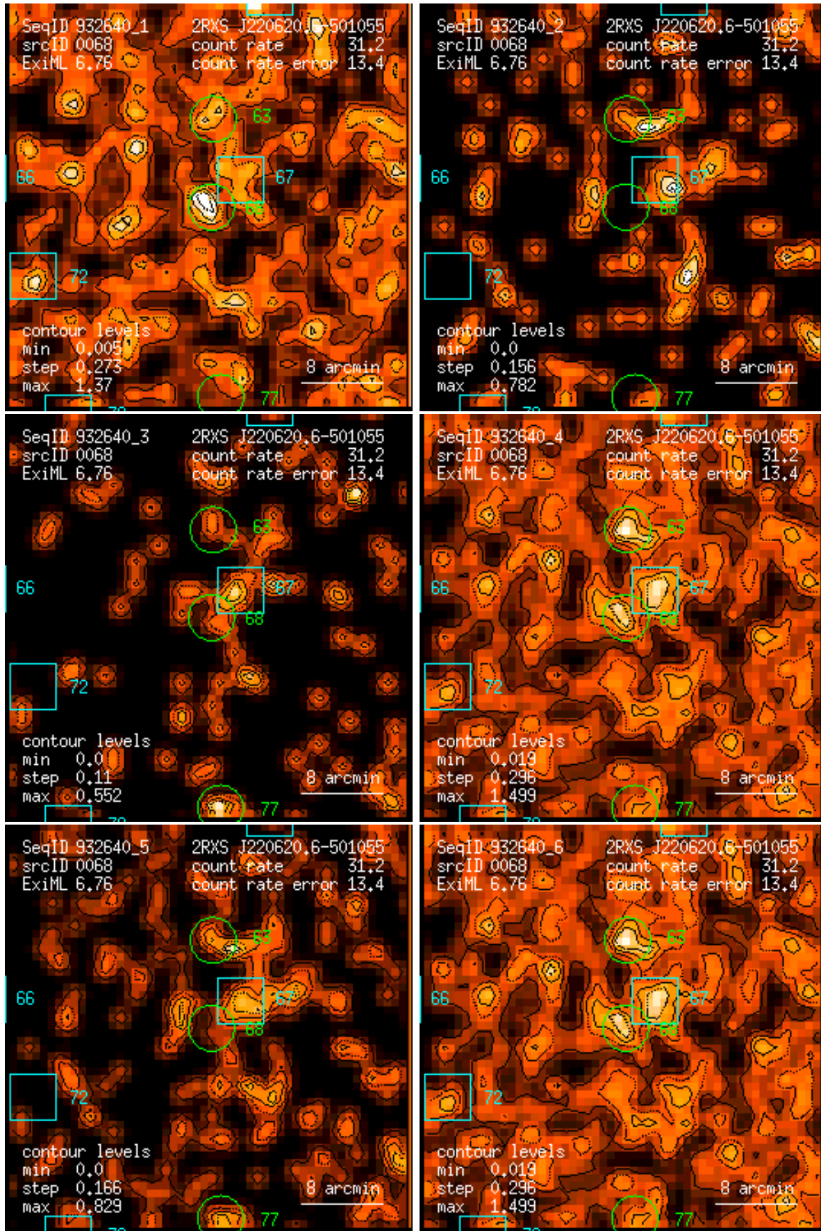
Figure 68: RASS 932640: detection 0068: band rate images, Gaussian filter: (1) PSPC channels 11 – 41, (2) 52 – 90, (3) 91 – 201, (4) 11 – 235, (5) 52 – 201, (6) 11 – 201. Broad band rates in counts/ks. Band rate contour levels in counts/ks/arcmin 2 .
